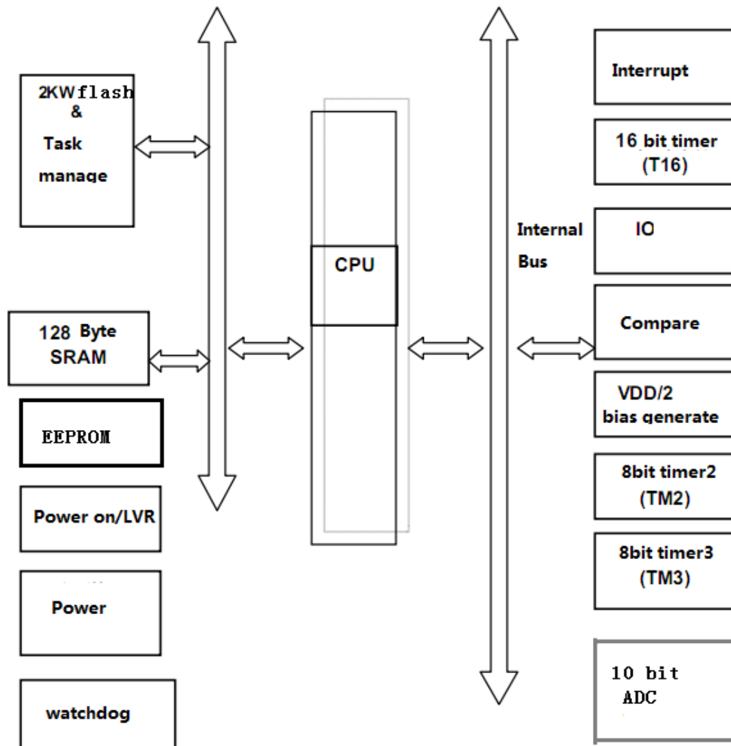
MCU block diagram
