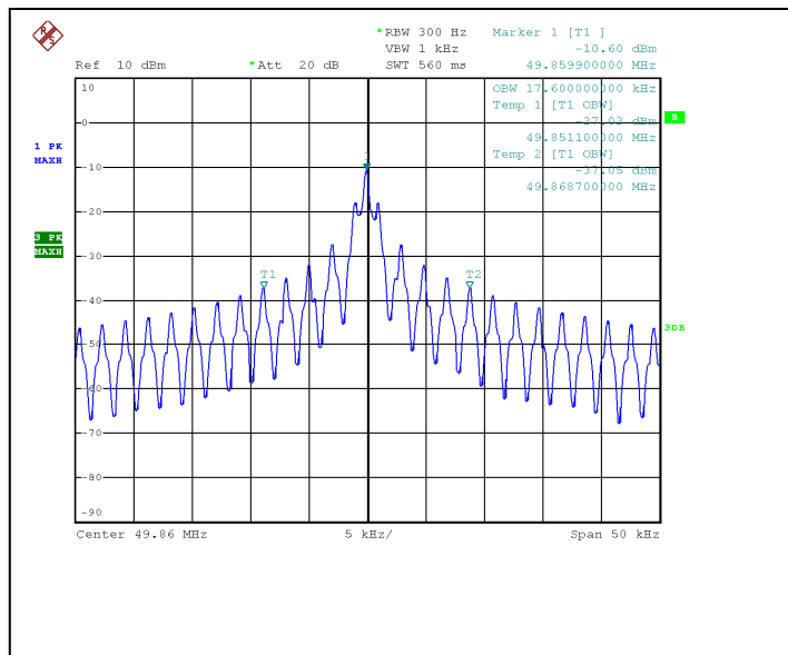
99% Bandwidth
