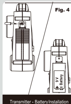
Transmitter - Battery Installation
