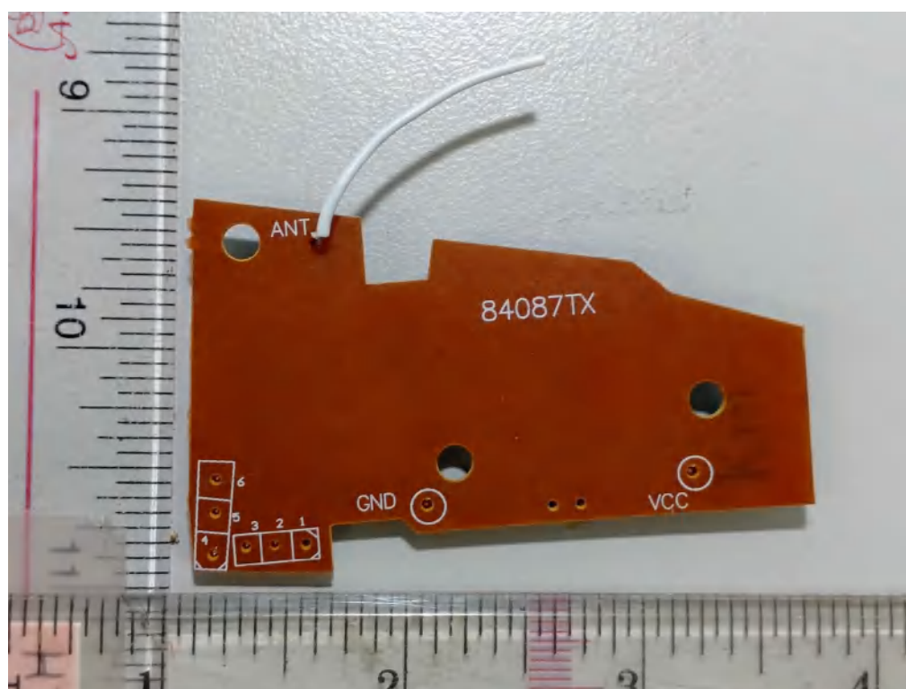
Internal View
