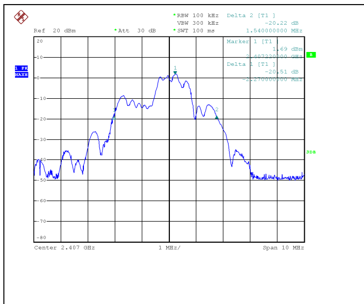
Channel: 2407MHz
