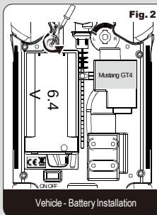
Vehicle - Battery Installation
