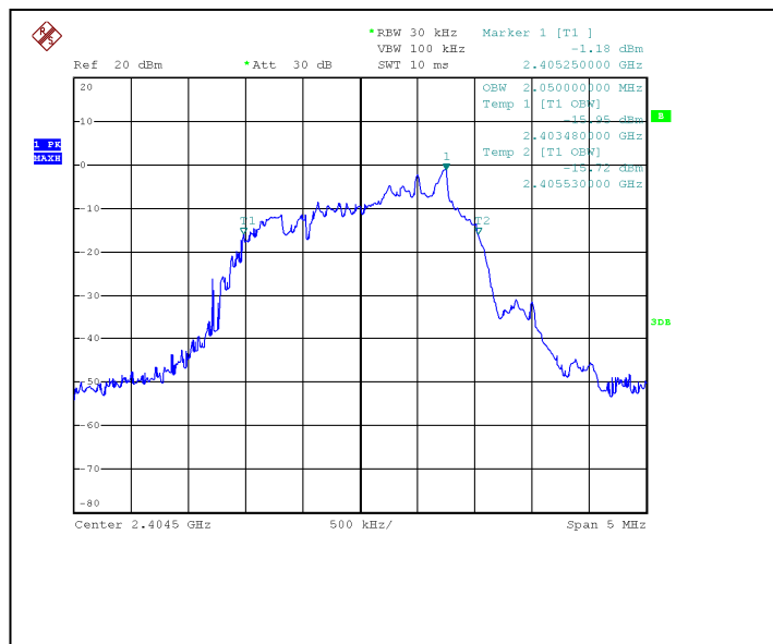
Channel: 2405MHz
