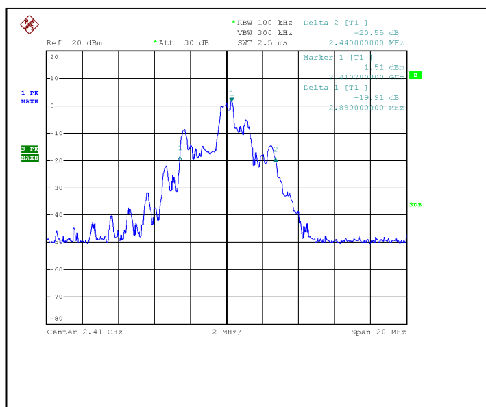
Channel: 2410MHz
