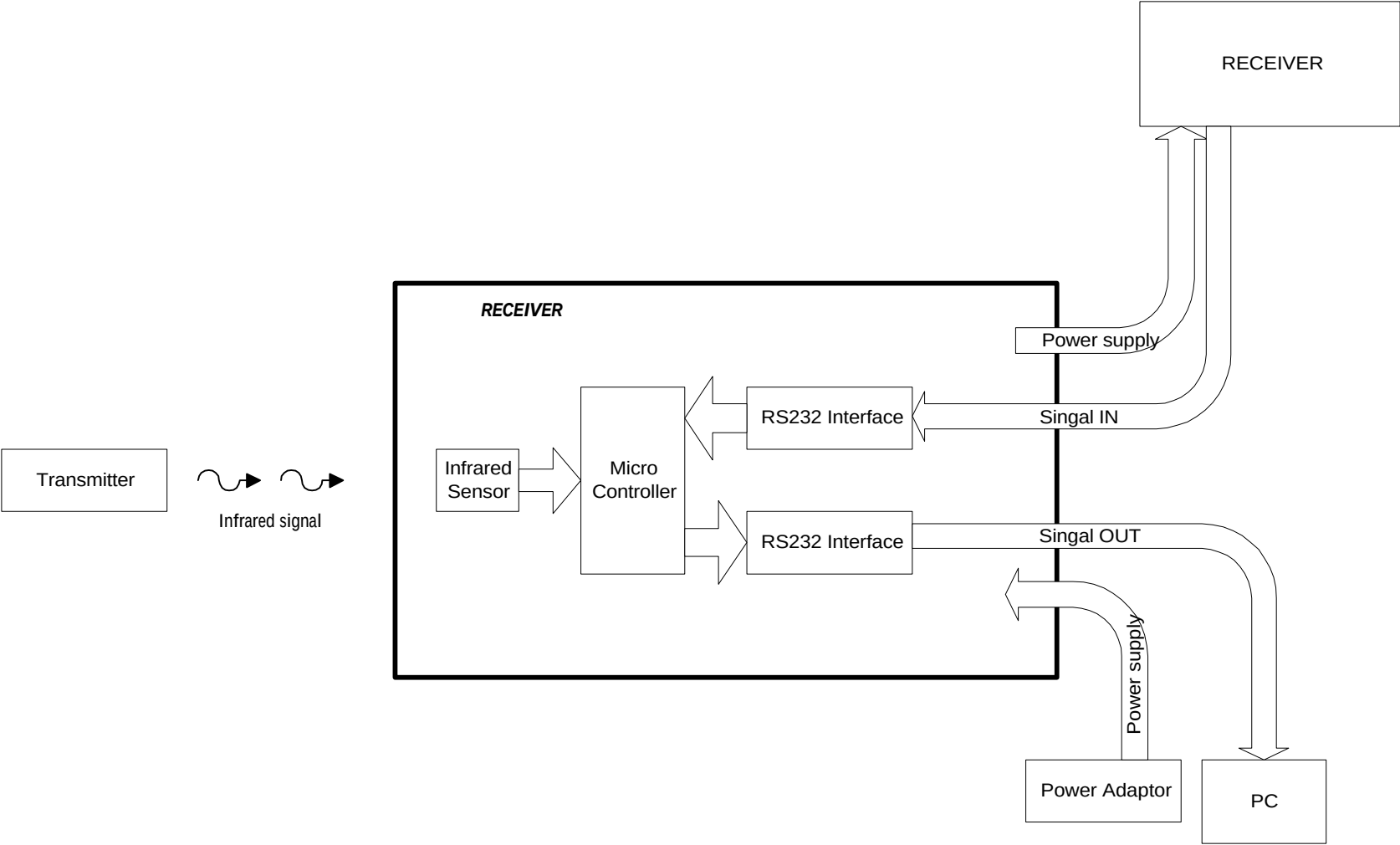
Block diagram of Receiver
