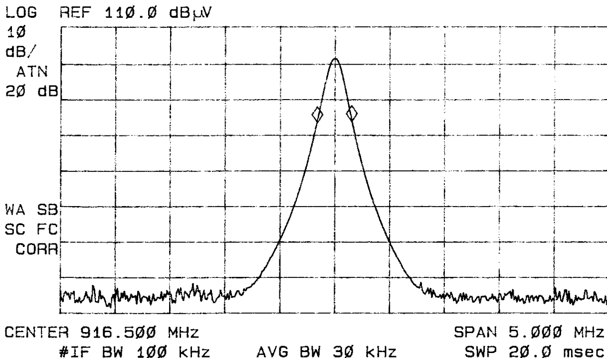
Figure 1 99.5% Power Occupied Bandwidth
