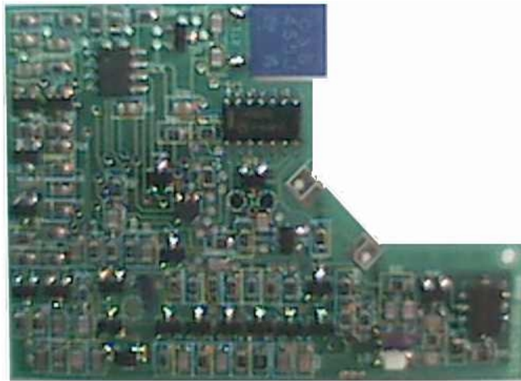
Asset Tag PCB - Bottom View
