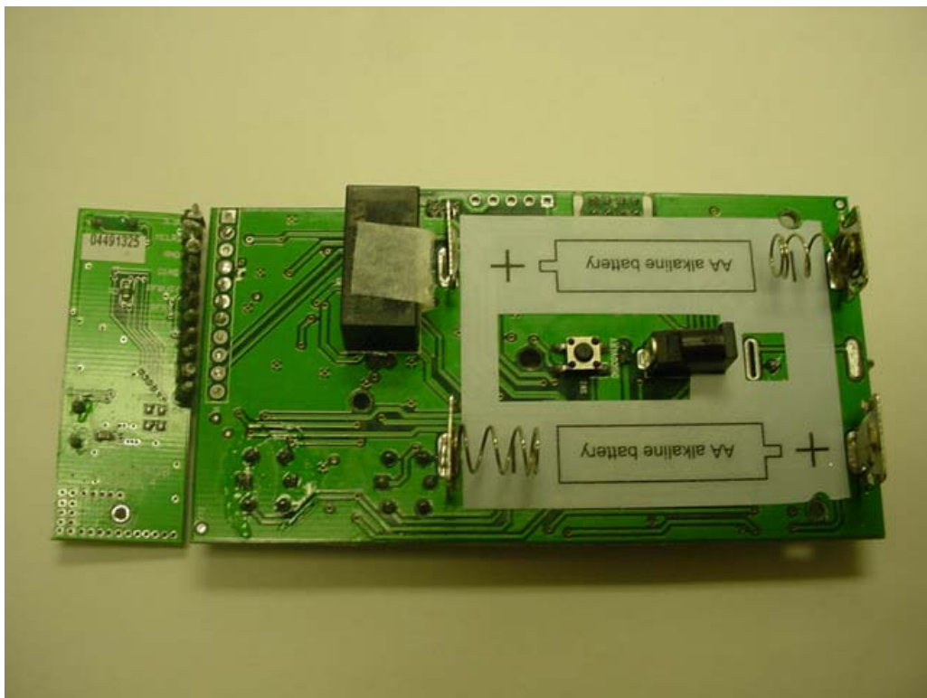
PCB Back
