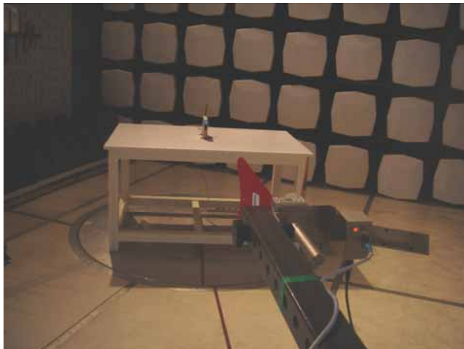
Radiation Emission Test View For 1GHz-5GHz
