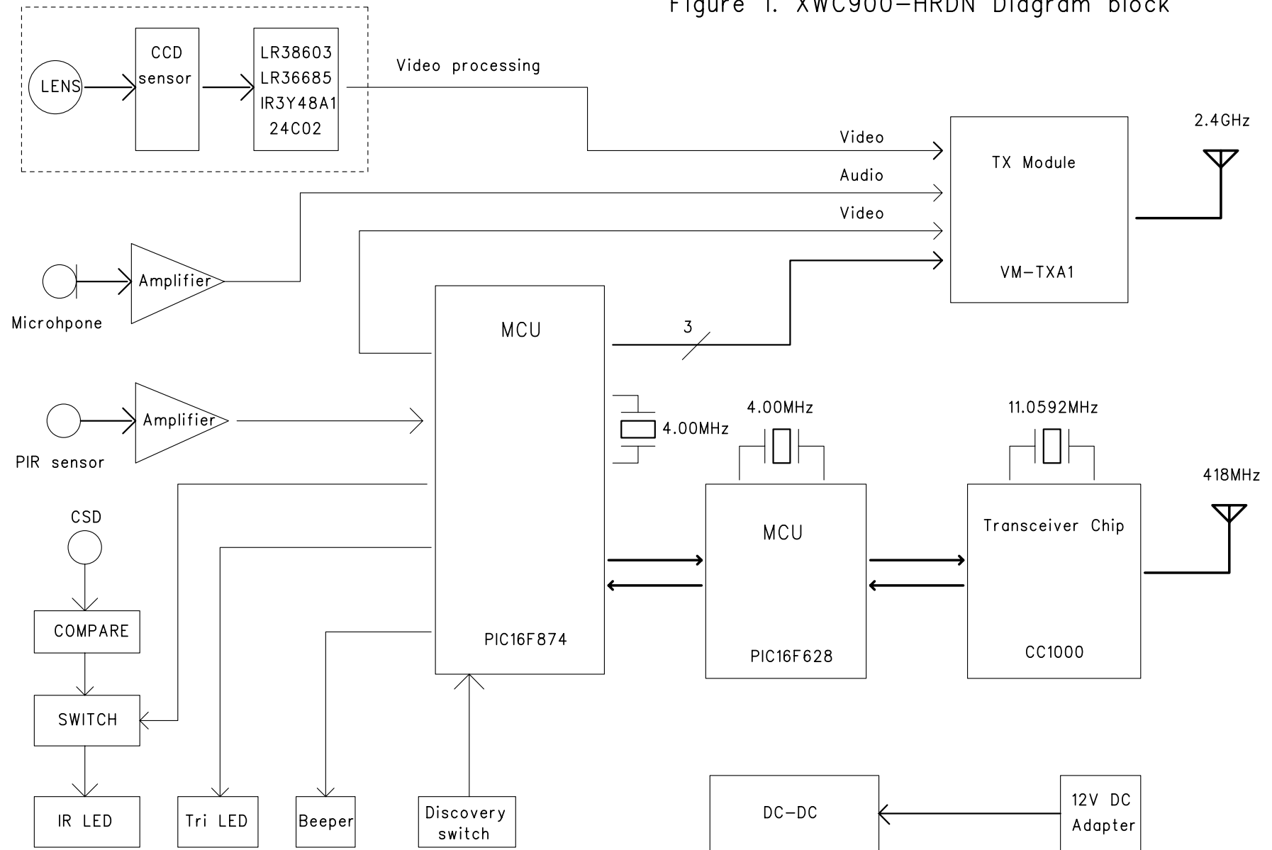
Figure 1. XWC900-HRDN Diagram block
