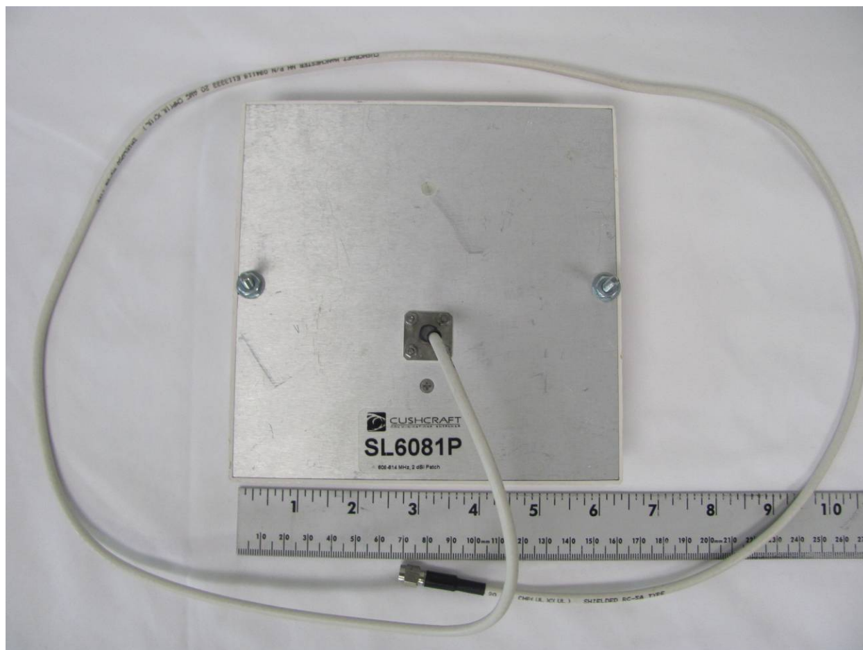
Figure 9. 2 dBi Patch Antenna, Bottom
