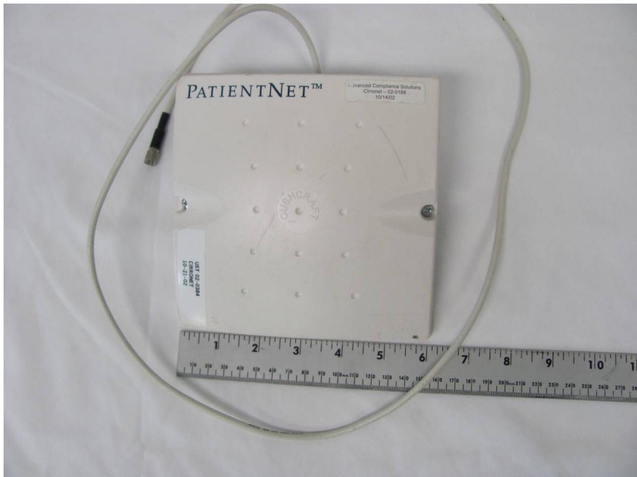
Figure 8. 2 dBi Patch Antenna, Top
