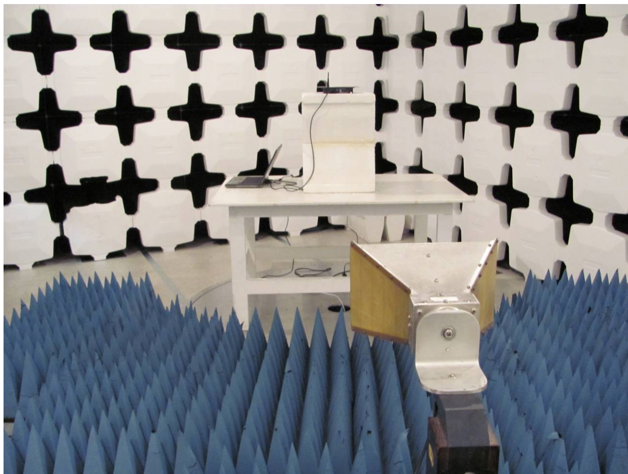
Figure 9. Radiated Emissions above 1 GHz
