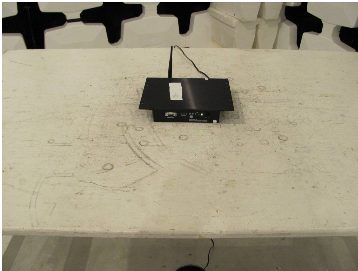
Figure 4. Radiated Emissions Measurements below 1 GHz (Both Dipole and Patch Antennas were tested using the same configuration)
