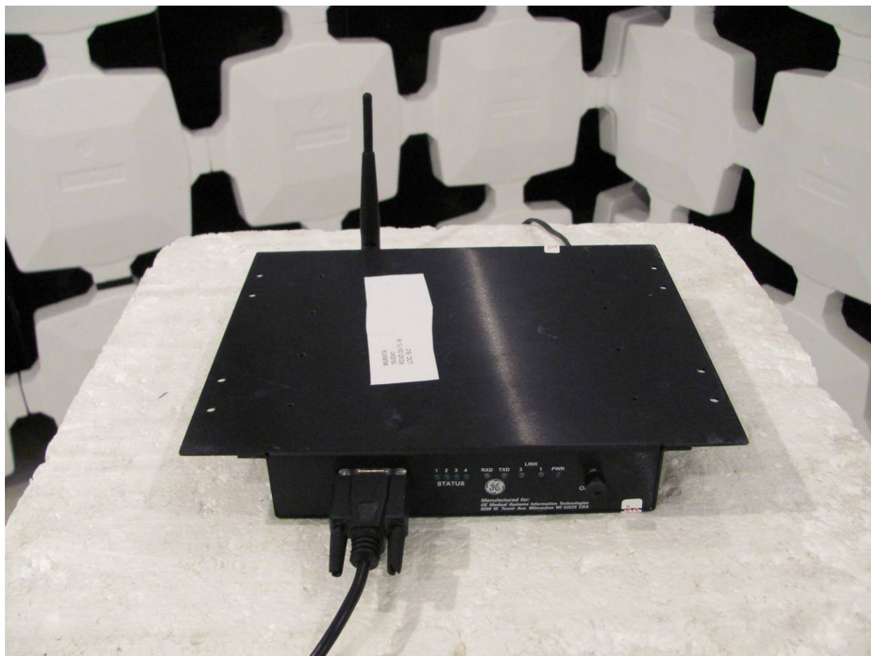
Figure 7. Radiated Emissions above 1 GHz (EUT placed on block elevated to 1.5 m test height)
