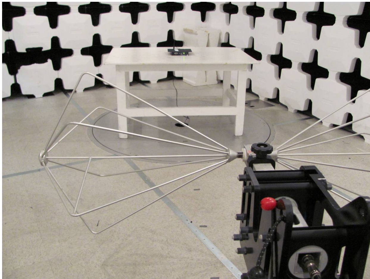
Figure 5. Radiated Emissions, 30 to 200 MHz
