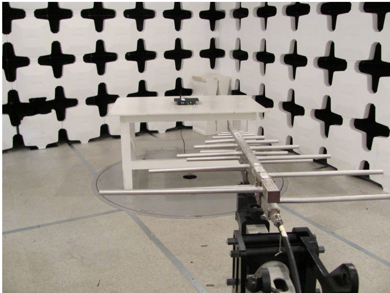
Figure 6. Radiated Emissions, 200 MHz to 1 GHz
