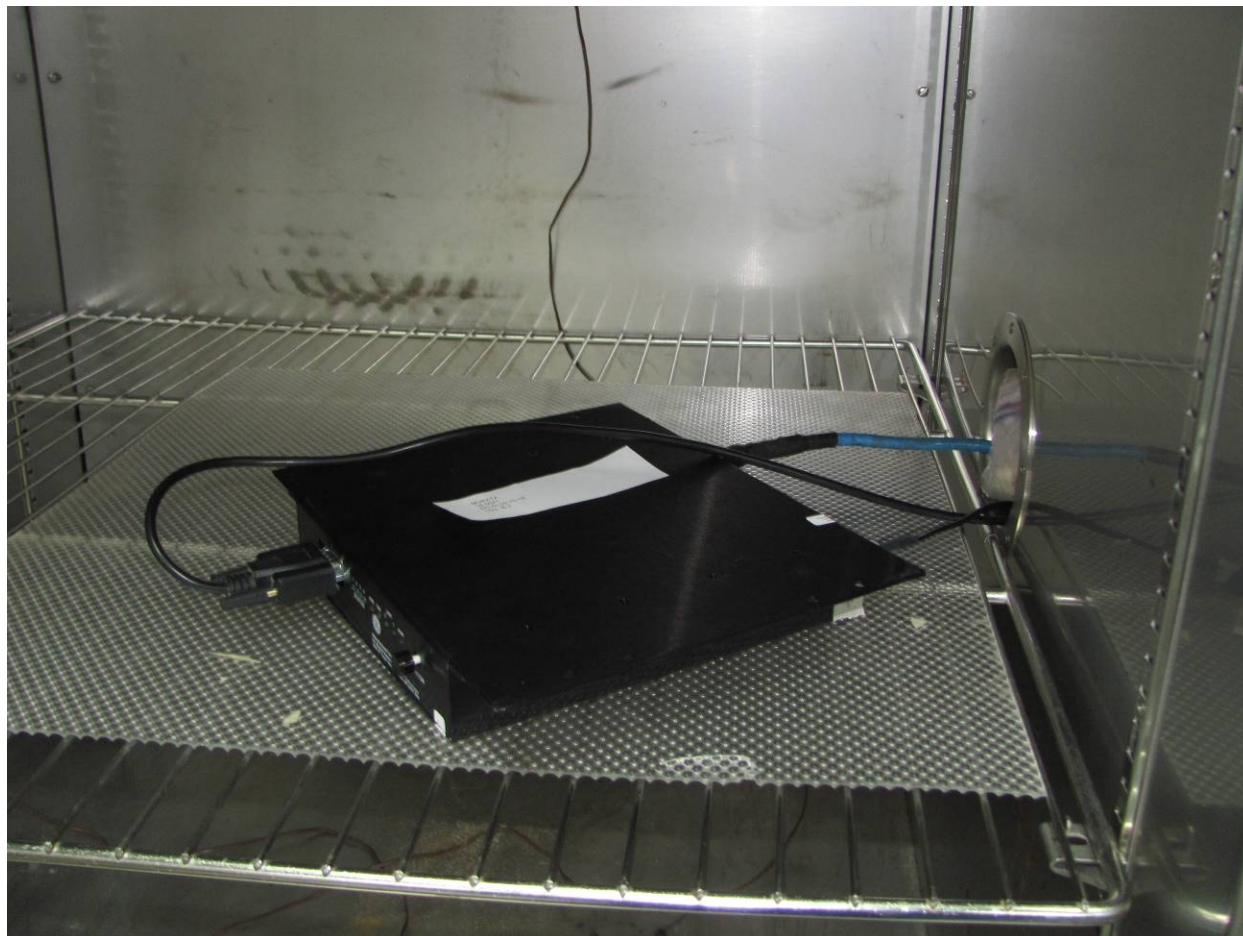
Figure 12. Temperature Testing Inside Chamber
