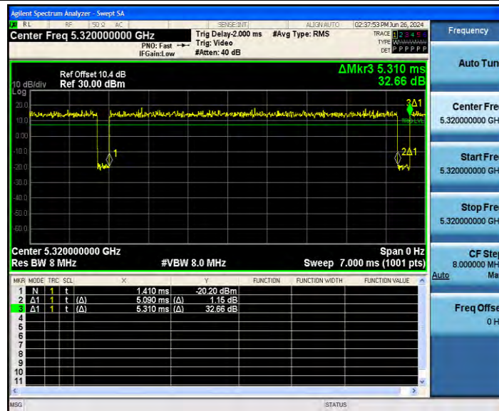
11N20SISO_Ant2_5320
