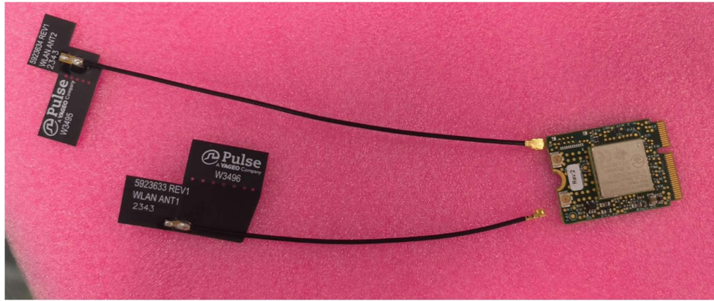
FPC Antenna type 1
