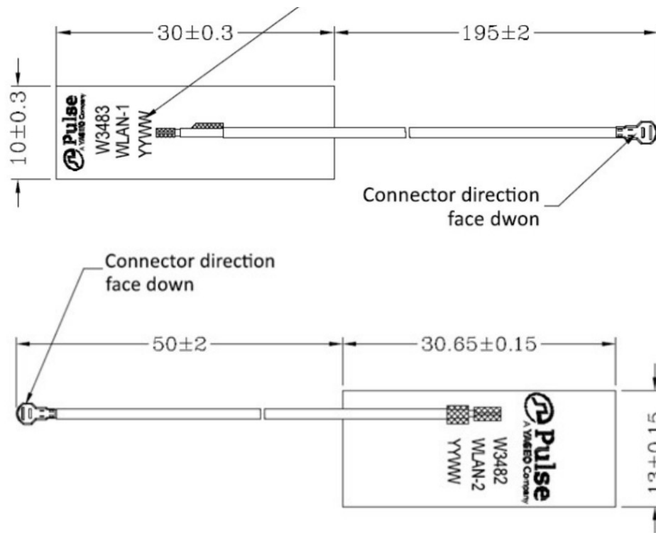
FPC Antenna type 2
