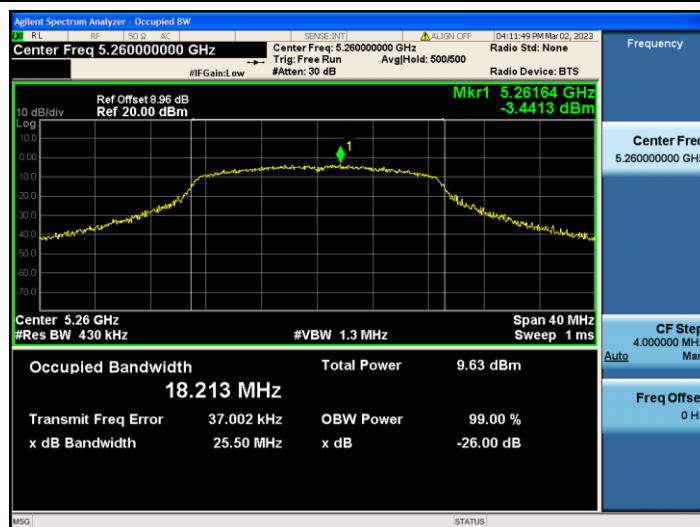
11N20SISO_Ant2_5260
