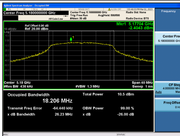
11N20SISO_Ant2_5180
