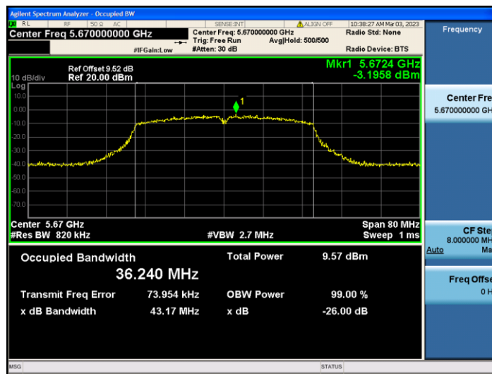
11N40SISO_Ant2_5670
