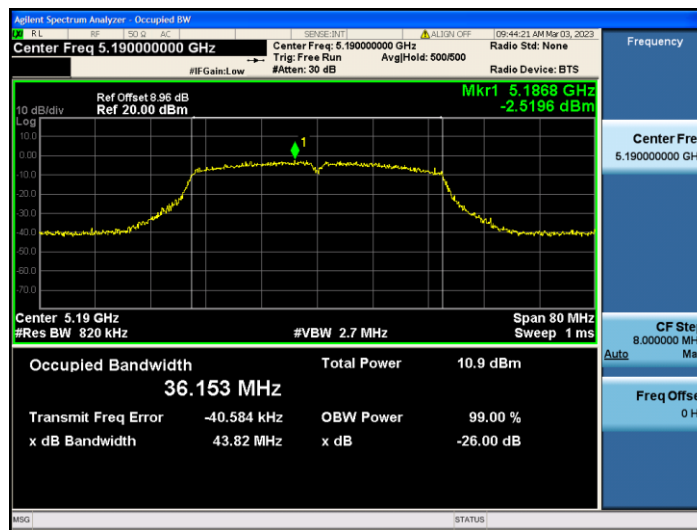
11N40SISO_Ant2_5190
