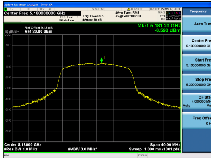
11A_Ant2_5180
