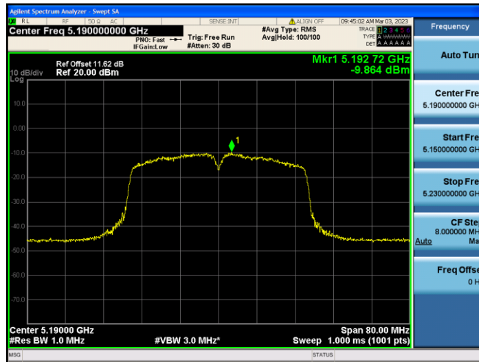
11N40SISO_Ant2_5190
