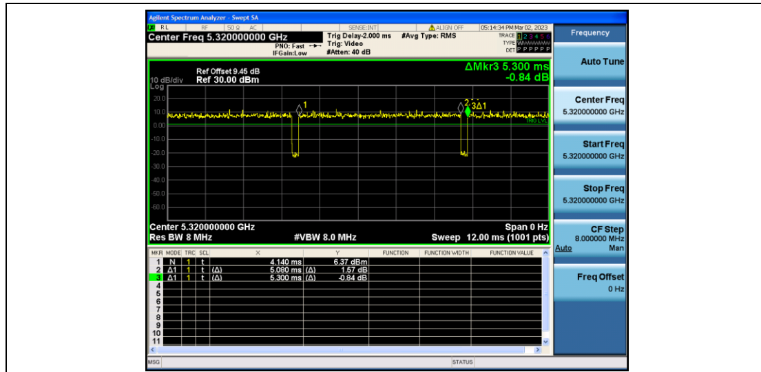
11N20SISO_Ant2_5320
