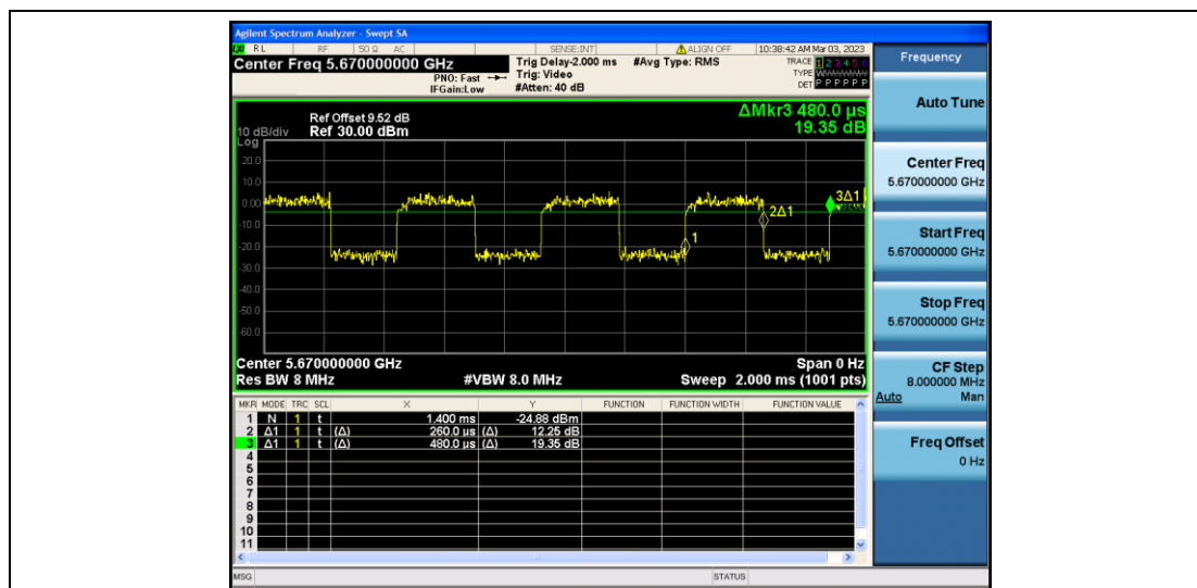
11N40SISO_Ant2_5670
