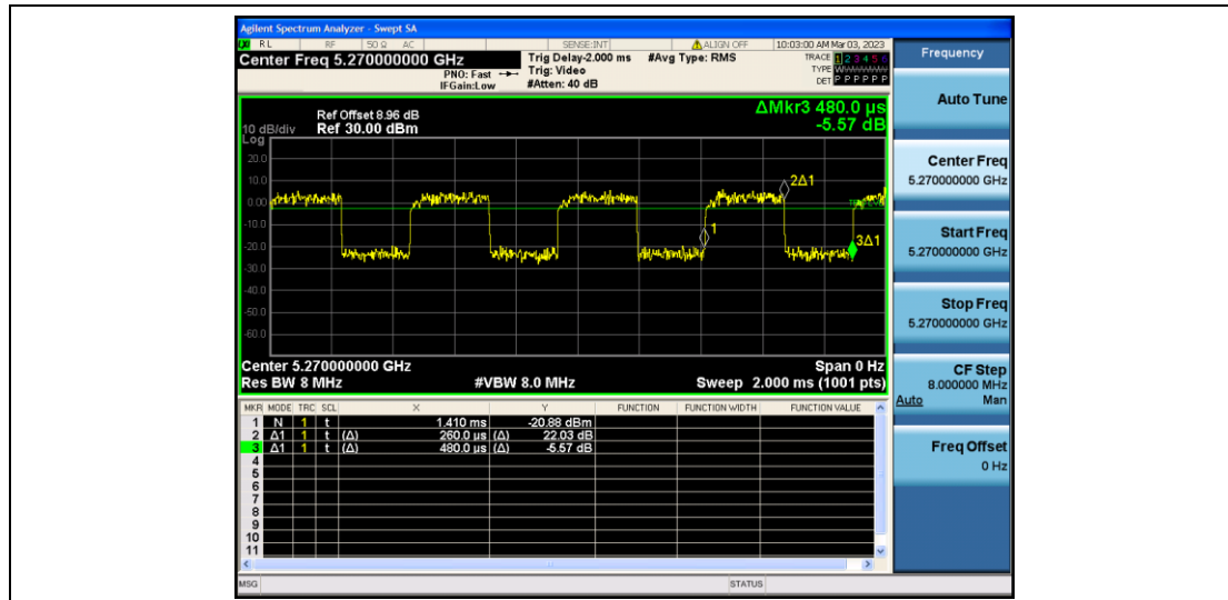
11N40SISO_Ant2_5270
