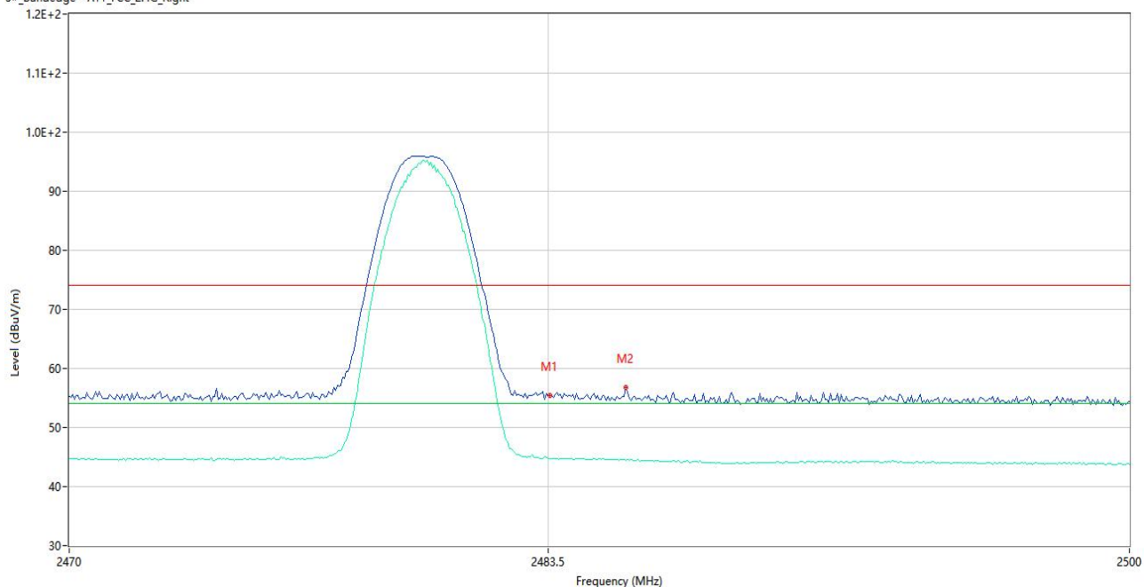
3#_Bandedge - ATT_FCC_2.4G_Right
