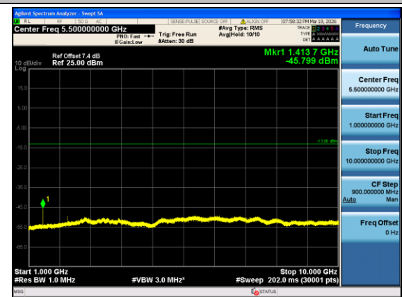
Band12-1.4MHz-16QAM-23095-1#0-1000-10000-PASS
