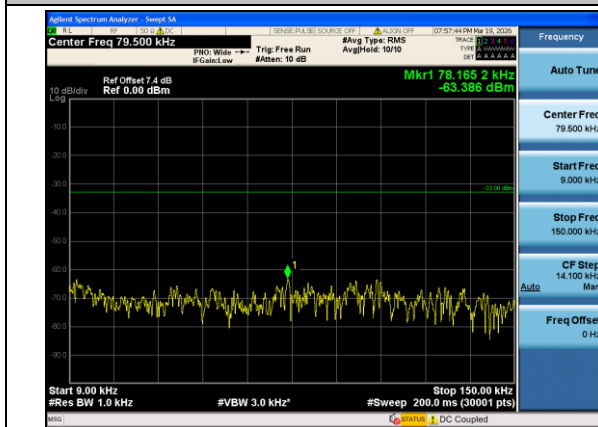
Band12-1.4MHz-QPSK-23095-1#0-0.009-0.15-PASS
