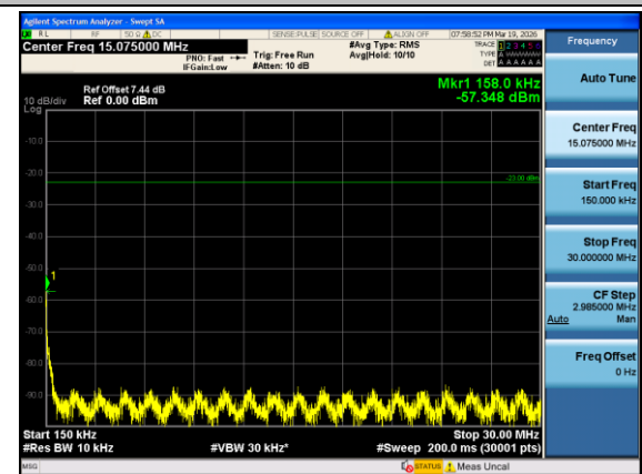
Band12-1.4MHz-QPSK-23173-1#5-0.15-30-PASS
