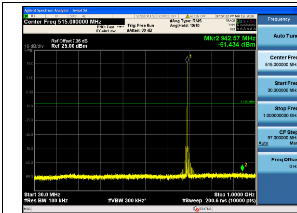
Band12-1.4MHz-16QAM-23017-1#0-30-1000-PASS
