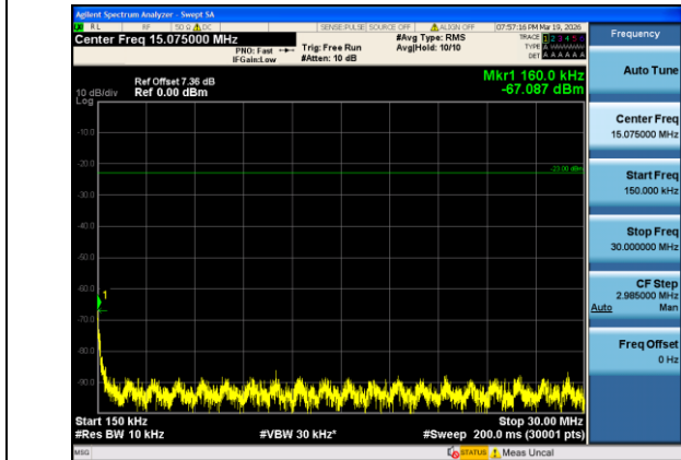
Band12-1.4MHz-QPSK-23017-1#0-0.15-30-PASS
