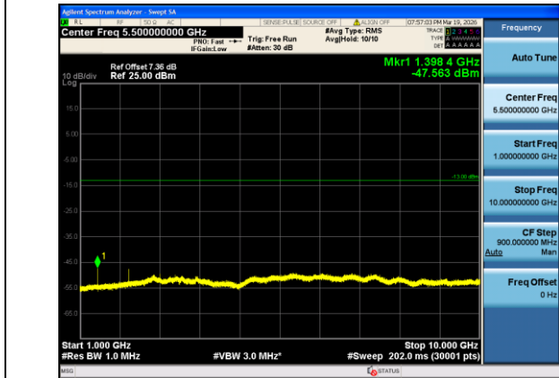
Band12-1.4MHz-QPSK-23017-1#0-1000-10000-PASS
