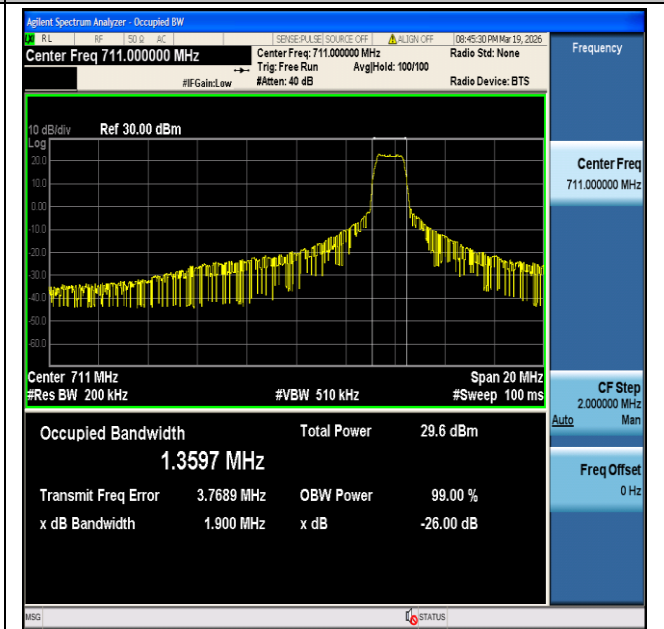
CatM1 Band12-10MHz-16QAM-23130-6#0-PASS
