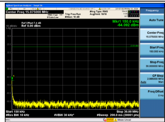
Band12-1.4MHz-QPSK-23095-1#0-0.15-30-PASS
