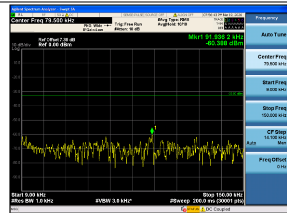
Band12-1.4MHz-QPSK-23017-1#0-0.009-0.15-PASS
