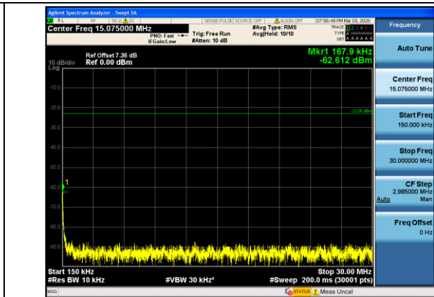
Band12-1.4MHz-QPSK-23017-1#0-0.15-30-PASS
