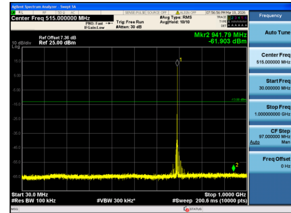
Band12-1.4MHz-QPSK-23017-1#0-30-1000-PASS
