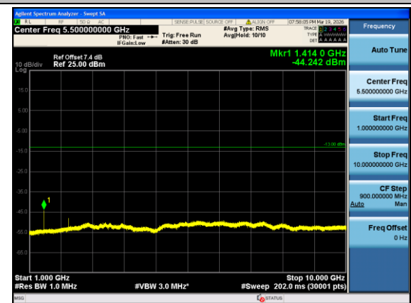
Band12-1.4MHz-QPSK-23095-1#0-1000-10000-PASS
