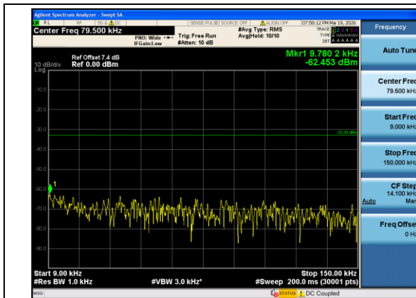
Band12-1.4MHz-16QAM-23095-1#0-0.009-0.15-PASS
