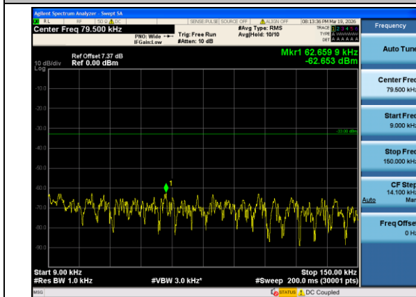
Band12-3MHz-16QAM-23025-1#0-0.009-0.15-PASS
