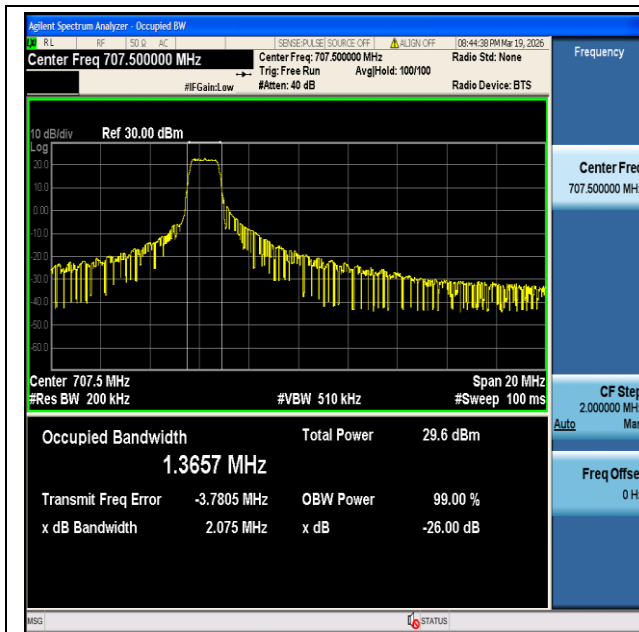
CatM1 Band12-10MHz-QPSK-23095-6#0-PASS
