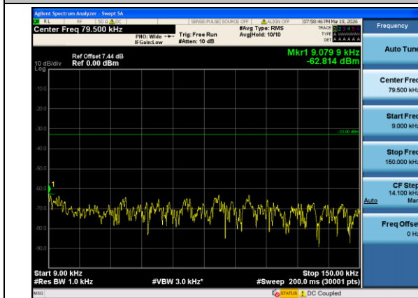
Band12-1.4MHz-QPSK-23173-1#5-0.009-0.15-PASS
