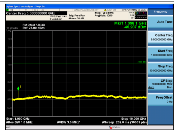
Band12-1.4MHz-16QAM-23017-1#0-1000-10000-PASS
