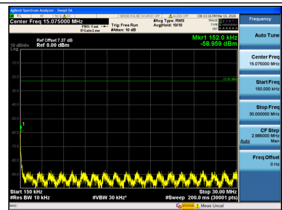
Band12-3MHz-QPSK-23025-1#0-0.15-30-PASS
