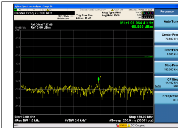
Band12-3MHz-QPSK-23025-1#0-0.009-0.15-PASS
