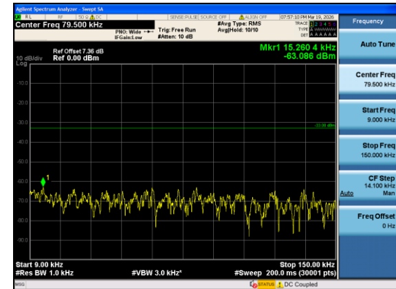
Band12-1.4MHz-QPSK-23017-1#0-0.009-0.15-PASS
