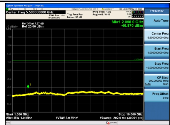
Band12-3MHz-QPSK-23025-1#0-1000-10000-PASS
