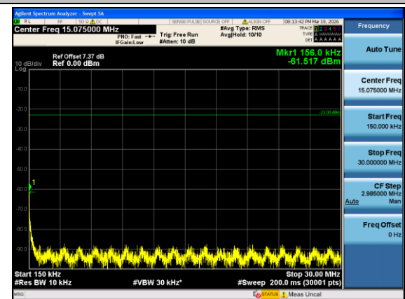
Band12-3MHz-16QAM-23025-1#0-0.15-30-PASS
