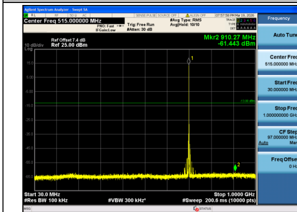
Band12-1.4MHz-QPSK-23095-1#0-30-1000-PASS
