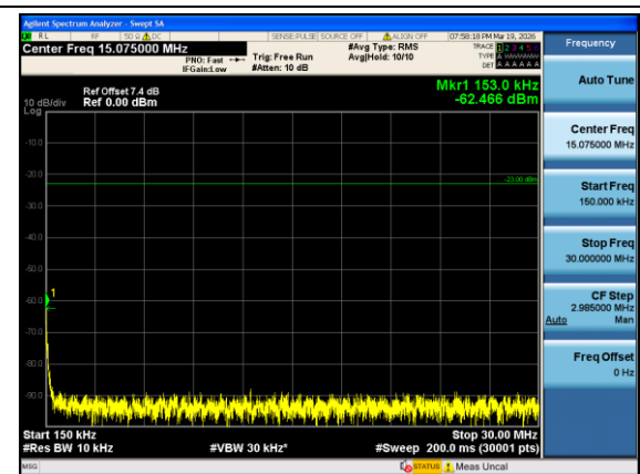
Band12-1.4MHz-16QAM-23095-1#0-0.15-30-PASS
