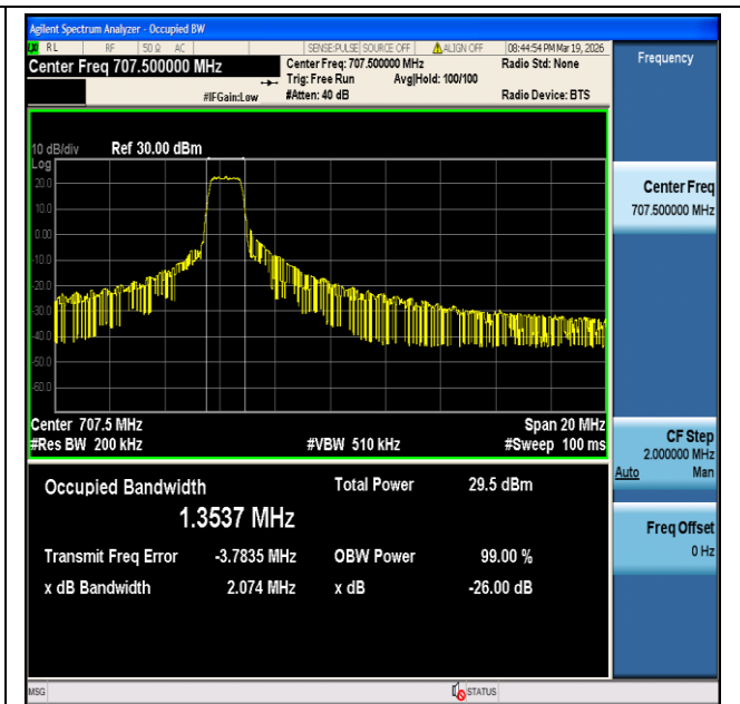
CatM1 Band12-10MHz-16QAM-23095-6#0-PASS
