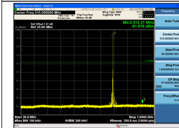
Band12-3MHz-QPSK-23025-1#0-30-1000-PASS
