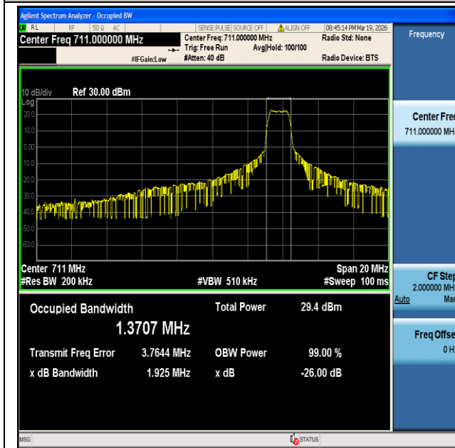
CatM1 Band12-10MHz-QPSK-23130-6#0-PASS
