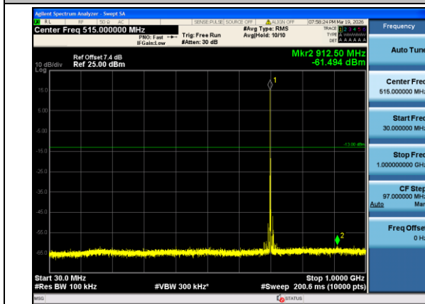
Band12-1.4MHz-16QAM-23095-1#0-30-1000-PASS
