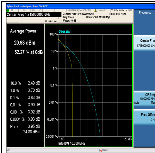
CatM1 Band4-10MHz-QPSK-20000-1#0-PASS
