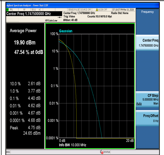
CatM1 Band4-15MHz-16QAM-20325-6#0-PASS
