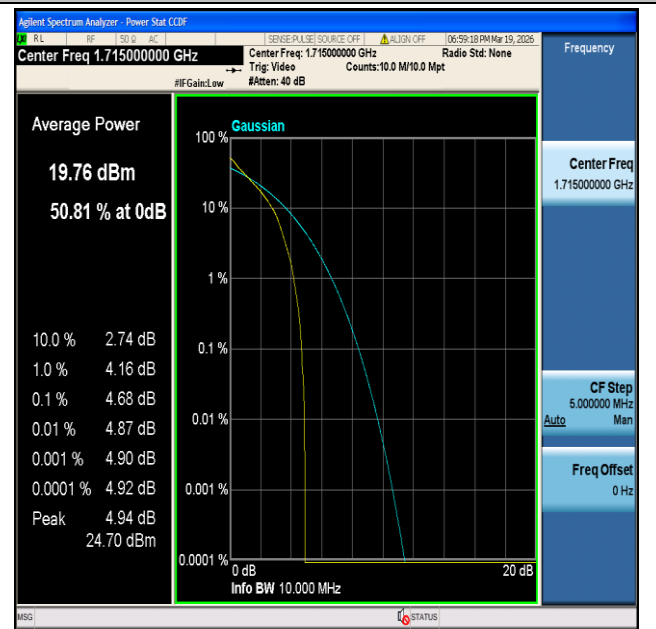
CatM1 Band4-10MHz-16QAM-20000-6#0-PASS
