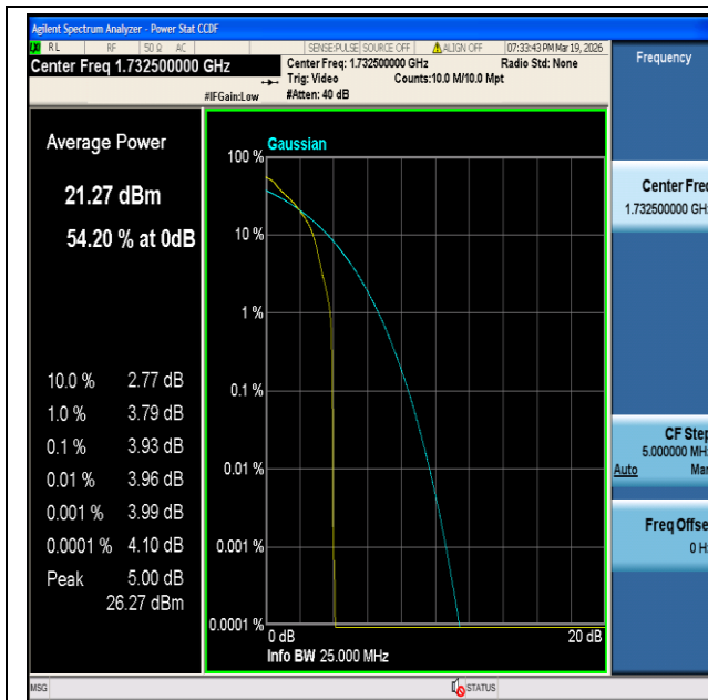
CatM1 Band4-20MHz-QPSK-20175-1#0-PASS
