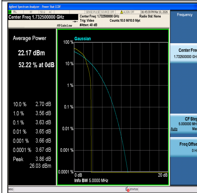
CatM1 Band4-5MHz-16QAM-20175-1#0-PASS
