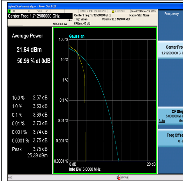
CatM1 Band4-5MHz-16QAM-19975-1#0-PASS
