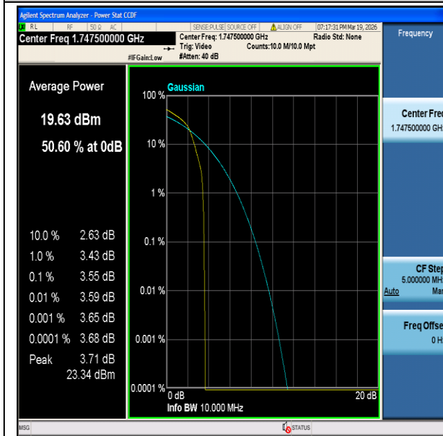
CatM1 Band4-15MHz-16QAM-20325-1#5-PASS
