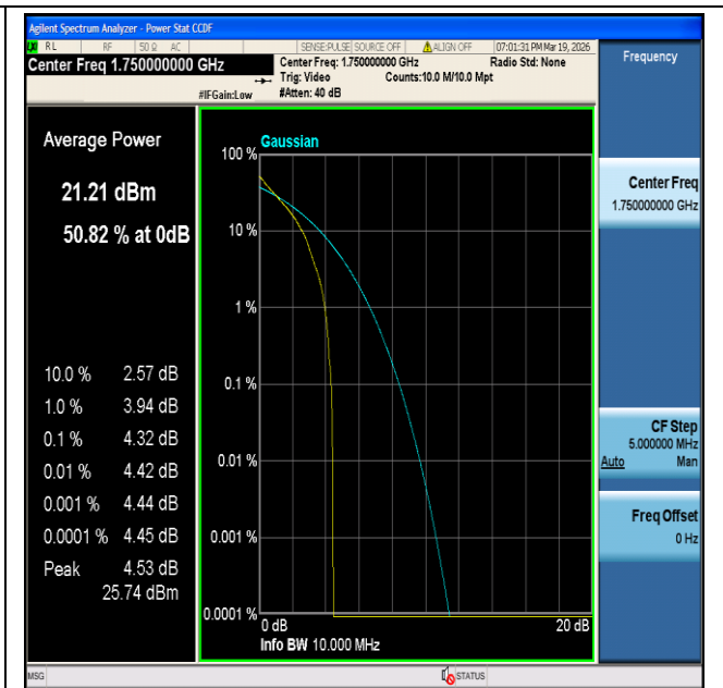
CatM1 Band4-10MHz-QPSK-20350-6#0-PASS
