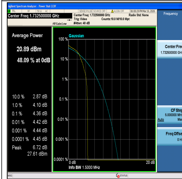
CatM1 Band4-1.4MHz-16QAM-20175-1#0-PASS
