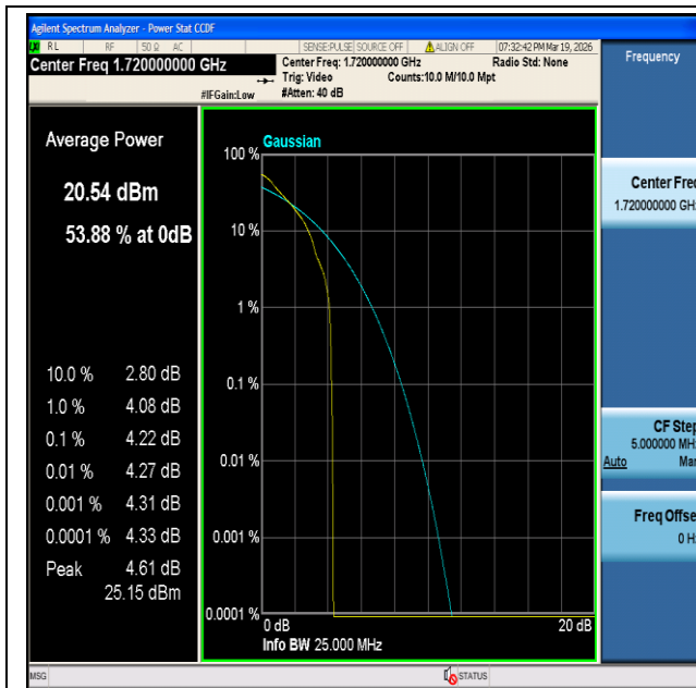
CatM1 Band4-20MHz-QPSK-20050-1#0-PASS
