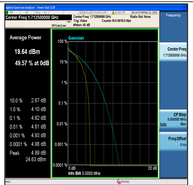
CatM1 Band4-5MHz-QPSK-19975-6#0-PASS
