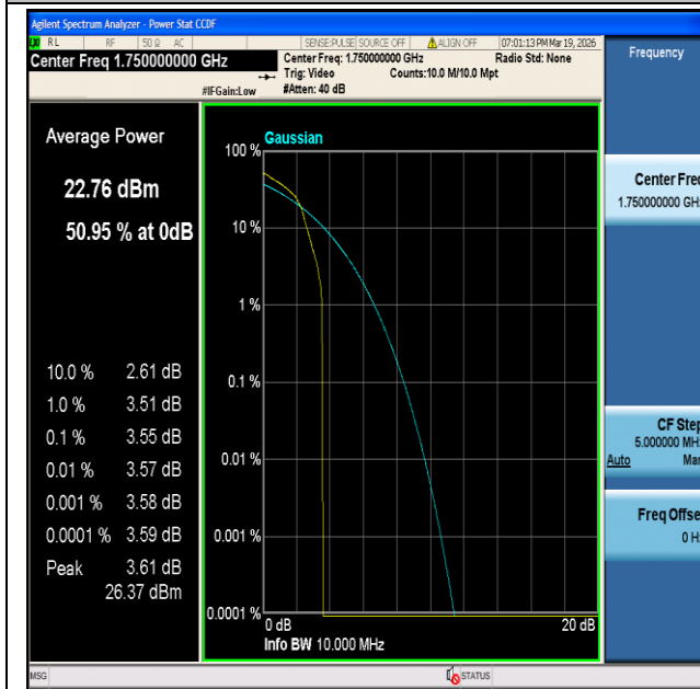
CatM1 Band4-10MHz-16QAM-20350-1#5-PASS
