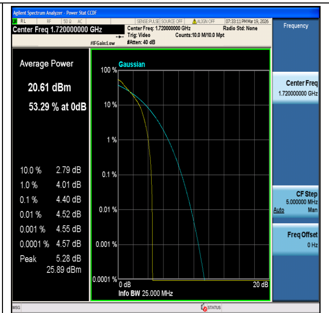
CatM1 Band4-20MHz-QPSK-20050-6#0-PASS
