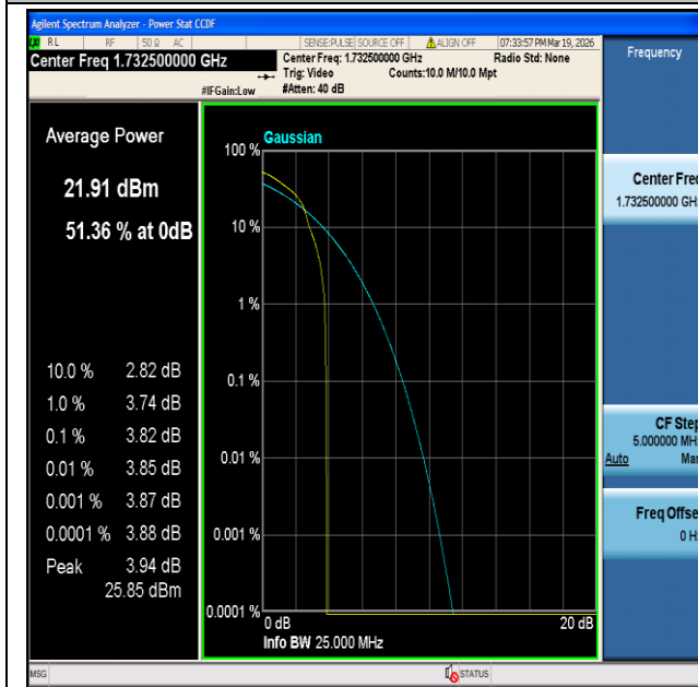
CatM1 Band4-20MHz-16QAM-20175-1#0-PASS
