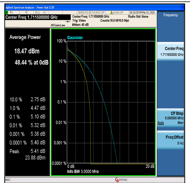
CatM1 Band4-3MHz-QPSK-19965-6#0-PASS
