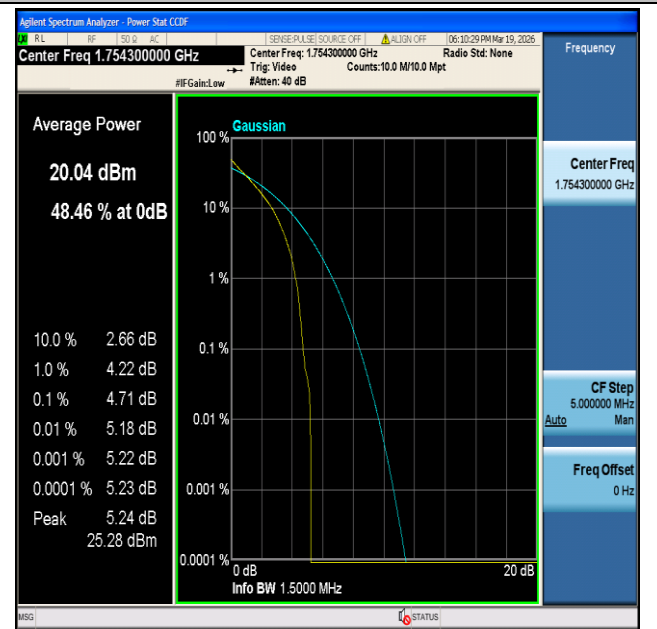
CatM1 Band4-1.4MHz-16QAM-20393-6#0-PASS
