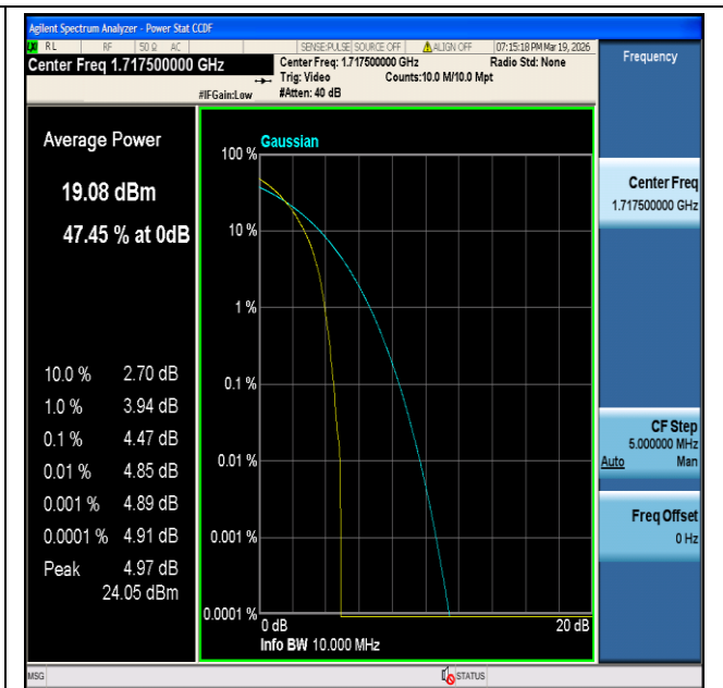
CatM1 Band4-15MHz-QPSK-20025-6#0-PASS
