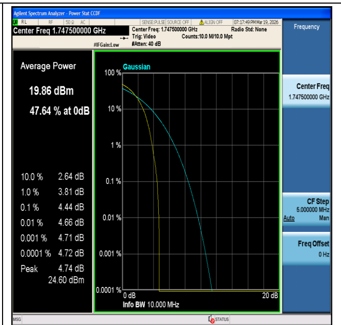
CatM1 Band4-15MHz-QPSK-20325-6#0-PASS
