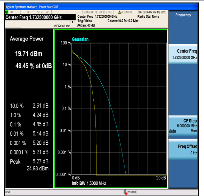
CatM1 Band4-1.4MHz-16QAM-20175-6#0-PASS
