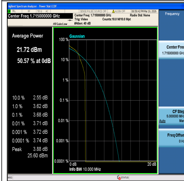
CatM1 Band4-10MHz-16QAM-20000-1#0-PASS
