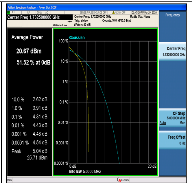
CatM1 Band4-5MHz-QPSK-20175-6#0-PASS
