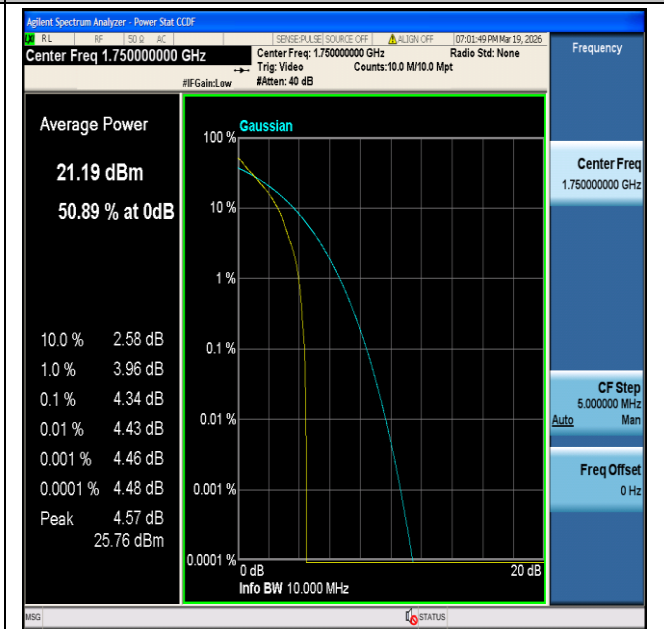
CatM1 Band4-10MHz-16QAM-20350-6#0-PASS
