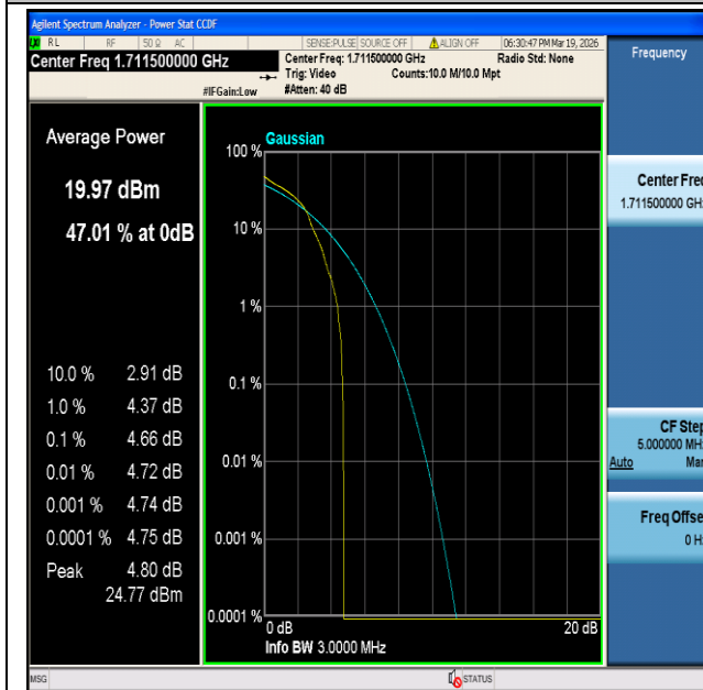
CatM1 Band4-3MHz-16QAM-19965-1#0-PASS
