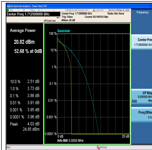
CatM1 Band4-5MHz-QPSK-19975-1#0-PASS
