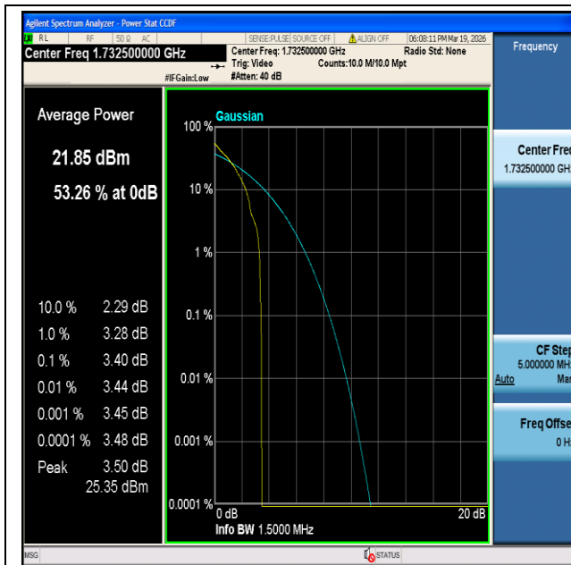
CatM1 Band4-1.4MHz-QPSK-20175-1#0-PASS
