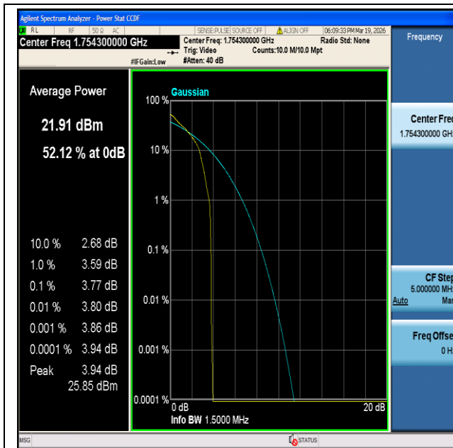
CatM1 Band4-1.4MHz-QPSK-20393-1#5-PASS
