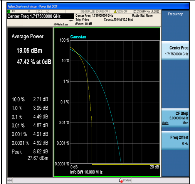
CatM1 Band4-15MHz-16QAM-20025-6#0-PASS
