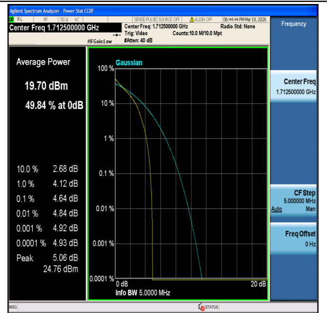
CatM1 Band4-5MHz-16QAM-19975-6#0-PASS
