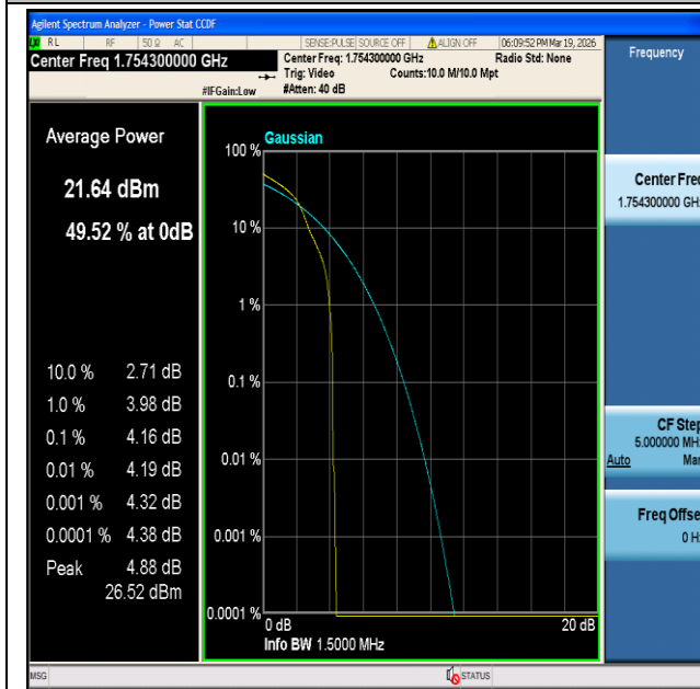
CatM1 Band4-1.4MHz-16QAM-20393-1#5-PASS
