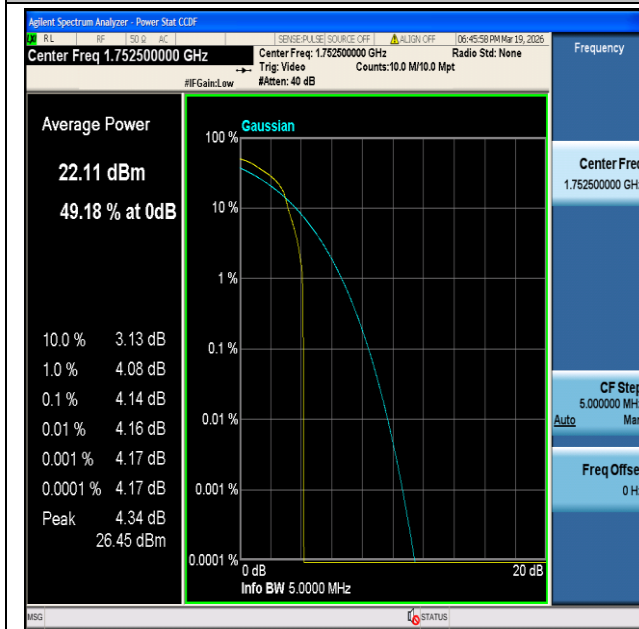
CatM1 Band4-5MHz-16QAM-20375-1#5-PASS
