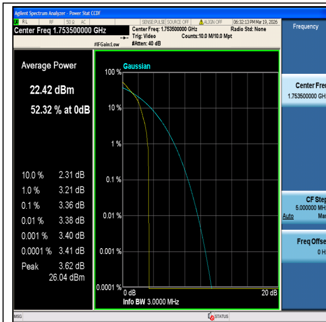
CatM1 Band4-3MHz-QPSK-20385-1#5-PASS
