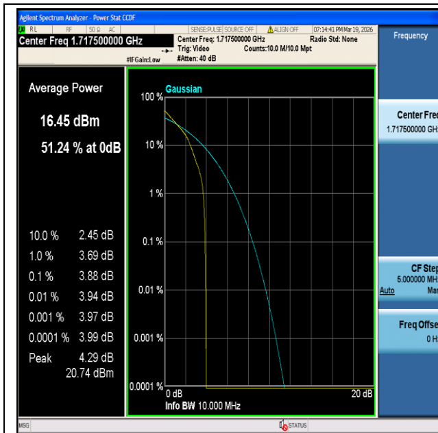
CatM1 Band4-15MHz-QPSK-20025-1#0-PASS
