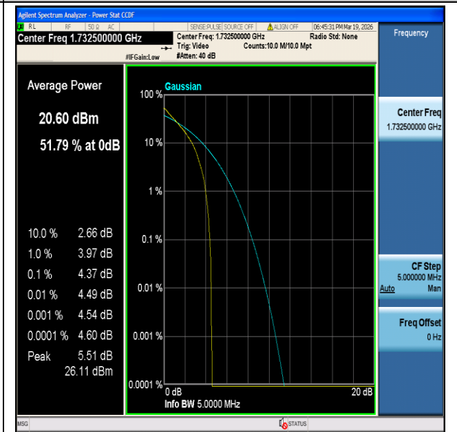
CatM1 Band4-5MHz-16QAM-20175-6#0-PASS
