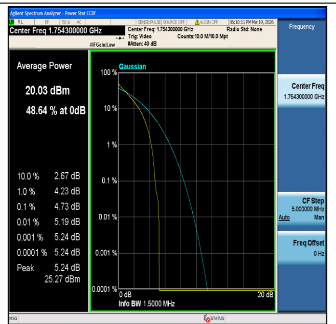
CatM1 Band4-1.4MHz-QPSK-20393-6#0-PASS
