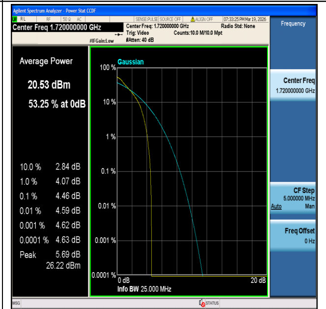
CatM1 Band4-20MHz-16QAM-20050-6#0-PASS
