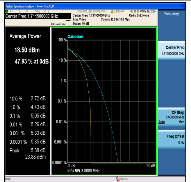
CatM1 Band4-3MHz-16QAM-19965-6#0-PASS
