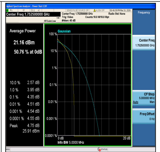
CatM1 Band4-5MHz-QPSK-20375-6#0-PASS
