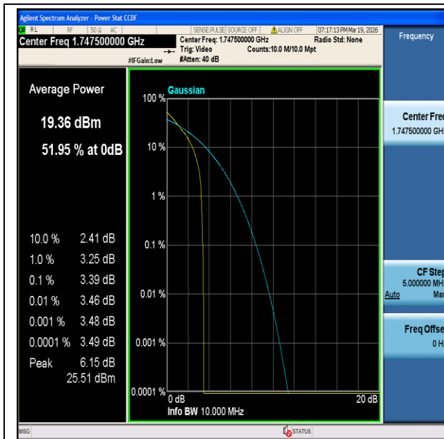
CatM1 Band4-15MHz-QPSK-20325-1#5-PASS
