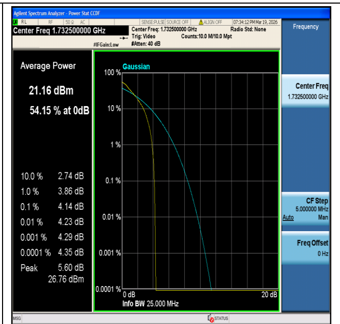
CatM1 Band4-20MHz-QPSK-20175-6#0-PASS
