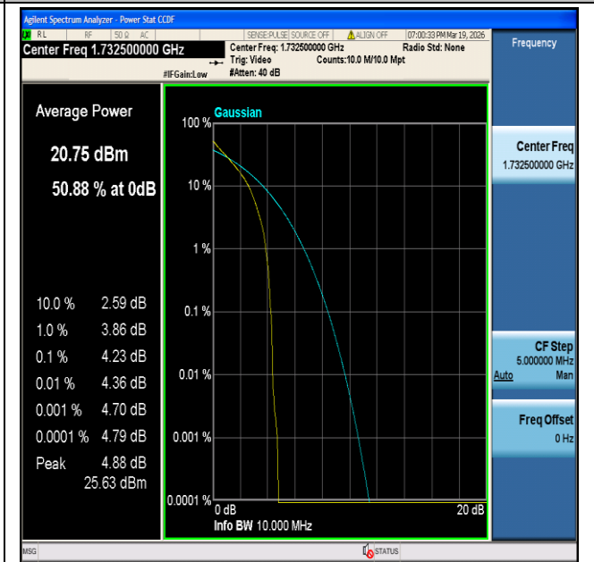
CatM1 Band4-10MHz-16QAM-20175-6#0-PASS
