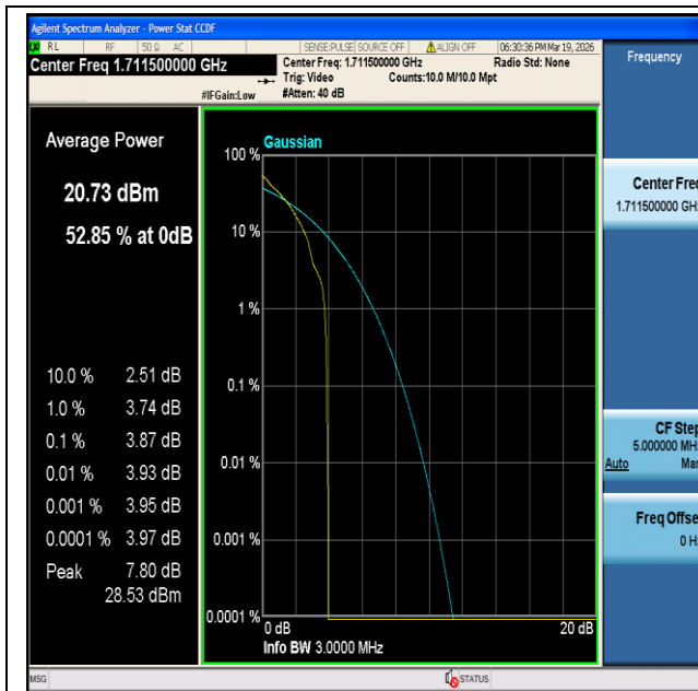
CatM1 Band4-3MHz-QPSK-19965-1#0-PASS
