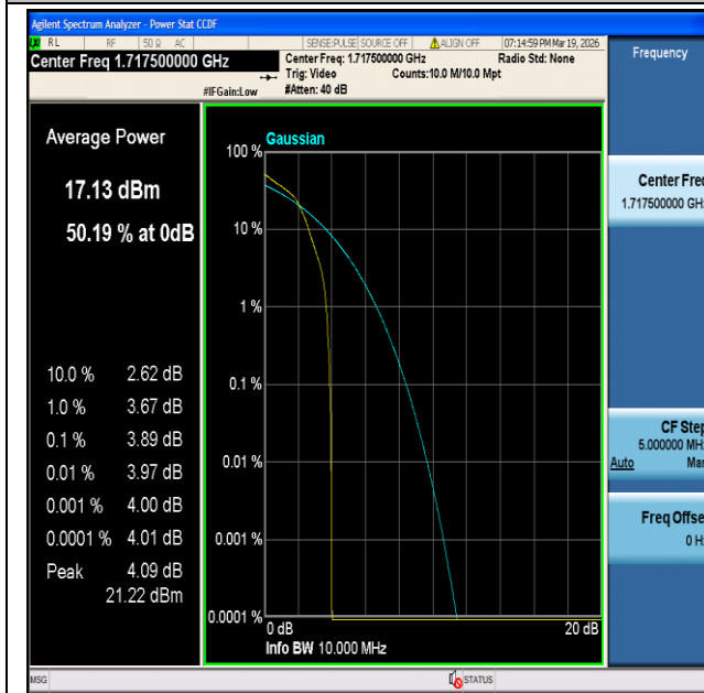
CatM1 Band4-15MHz-16QAM-20025-1#0-PASS
