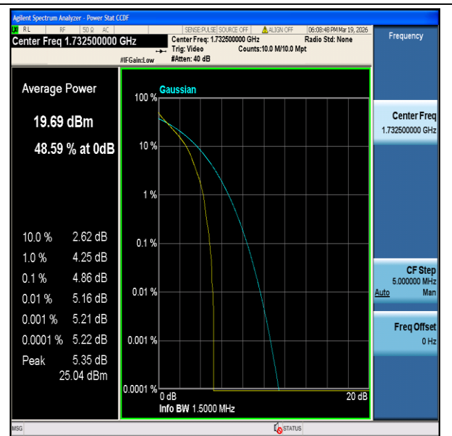
CatM1 Band4-1.4MHz-QPSK-20175-6#0-PASS
