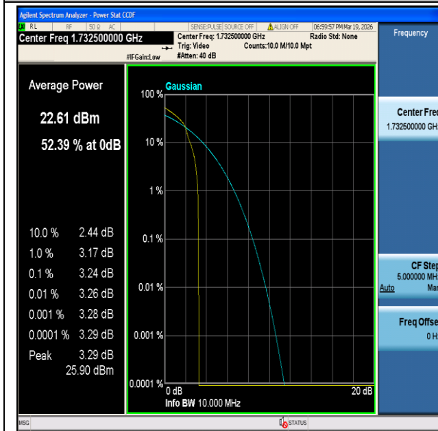
CatM1 Band4-10MHz-16QAM-20175-1#0-PASS
