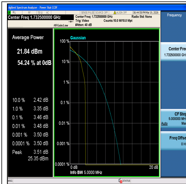
CatM1 Band4-5MHz-QPSK-20175-1#0-PASS
