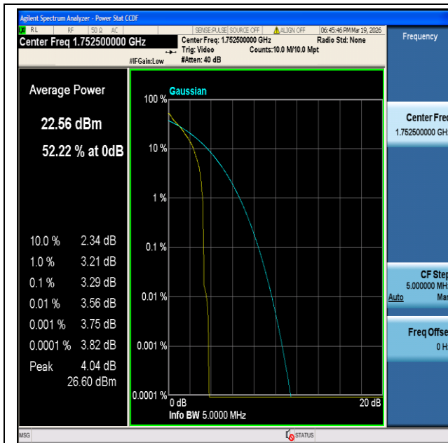
CatM1 Band4-5MHz-QPSK-20375-1#5-PASS
