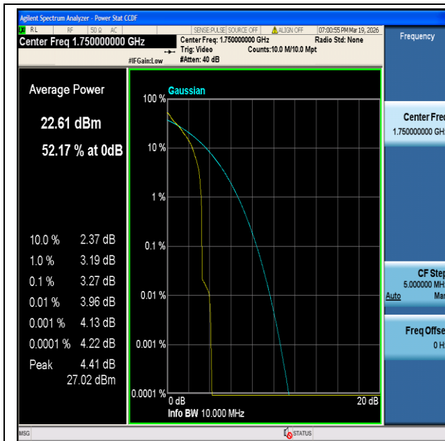
CatM1 Band4-10MHz-QPSK-20350-1#5-PASS
