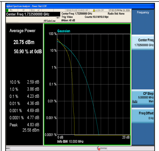
CatM1 Band4-10MHz-QPSK-20175-6#0-PASS
