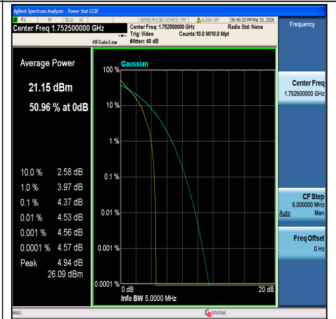
CatM1 Band4-5MHz-16QAM-20375-6#0-PASS
