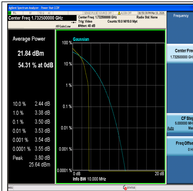
CatM1 Band4-10MHz-QPSK-20175-1#0-PASS
