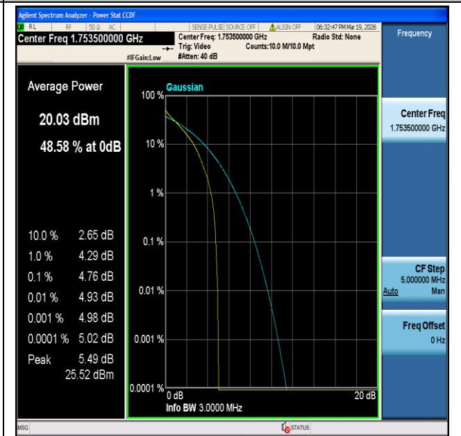
CatM1 Band4-3MHz-16QAM-20385-6#0-PASS
