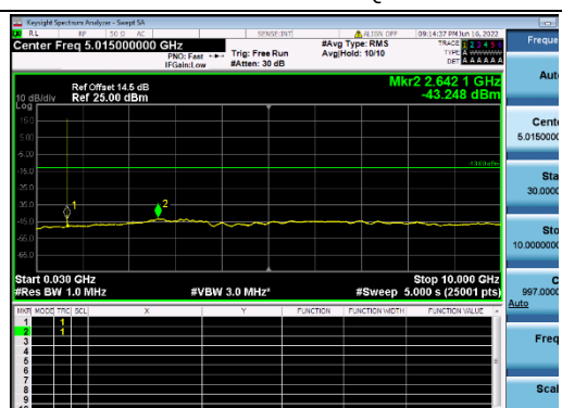
B12-10M-Mid CH-CSE-1-QPSK-1 RB 0
