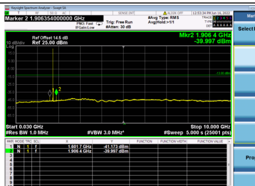
B4-15M-High CH-CSE-2-QPSK-1 RB 0
