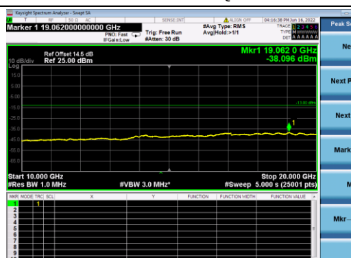
B4-20M-Mid CH-CSE-1-QPSK-1 RB 0
