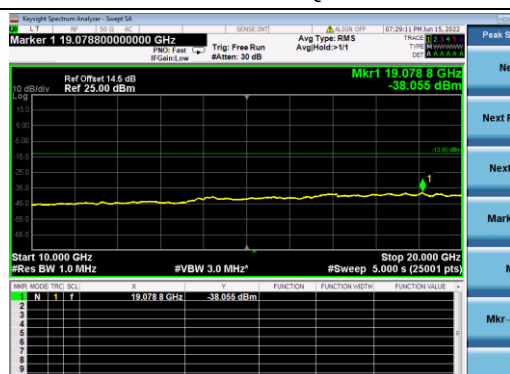
B4-3M-Mid CH-CSE-1-QPSK-1 RB 0
