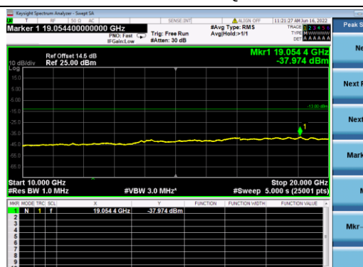
B4-10M-Mid CH-CSE-2-QPSK-1 RB 0
