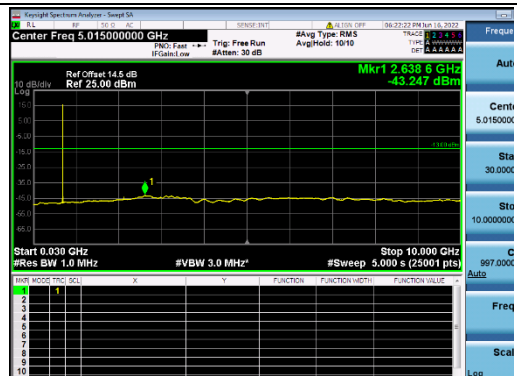
B12-1.4M-Low CH-CSE-1-QPSK-1 RB 0
