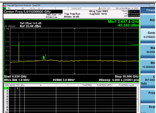
B12-1.4M-Mid CH-CSE-1-QPSK-1 RB 0
