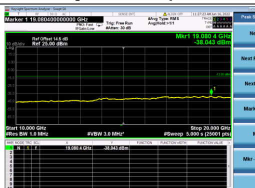
B4-10M-Low CH-CSE-1-QPSK-1 RB 0
