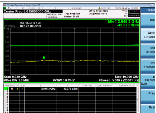
B12-10M-Low CH-CSE-1-QPSK-1 RB 0
