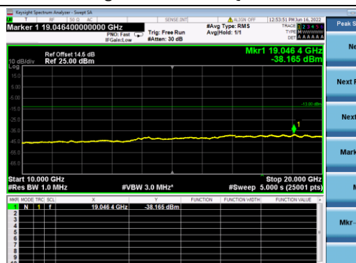
B4-15M-Low CH-CSE-1-QPSK-1 RB 0
