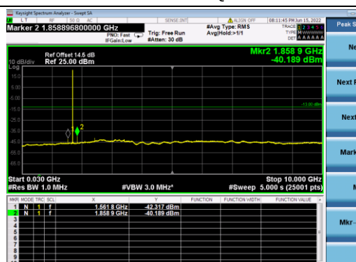
B4-5M-Low CH-CSE-1-QPSK-1 RB 0
