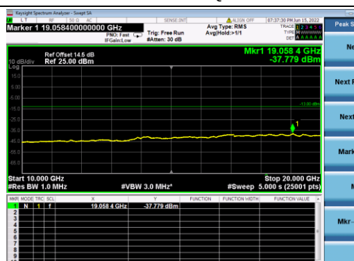
B4-3M-Mid CH-CSE-2-QPSK-1 RB 0
