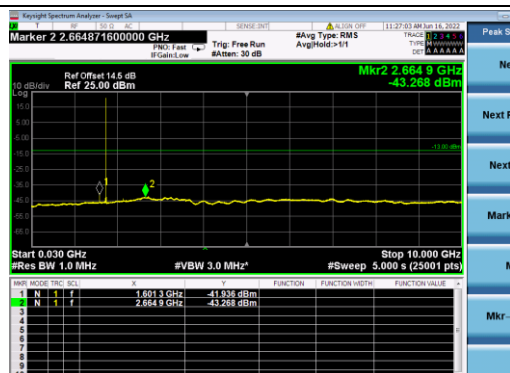
B4-10M-High CH-CSE-2-QPSK-1 RB 0
