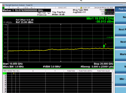
B4-20M-Mid CH-CSE-2-QPSK-1 RB 0
