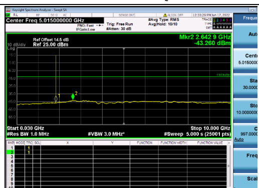
B25-5M-Low CH-CSE-2-QPSK-1 RB 0
