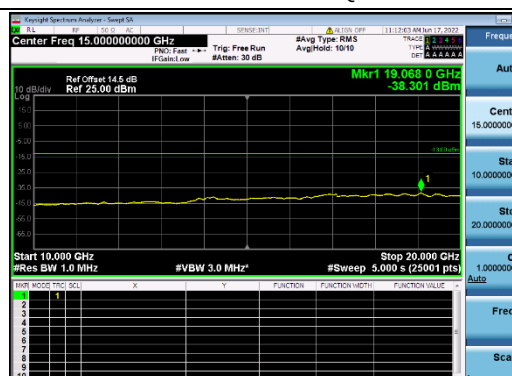
B25-3M-High CH-CSE-1-QPSK-1 RB 0
