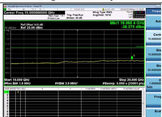
B25-10M-High CH-CSE-2-QPSK-1 RB 0
