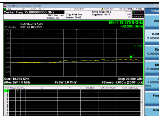
B25-10M-Mid CH-CSE-1-QPSK-1 RB 0
