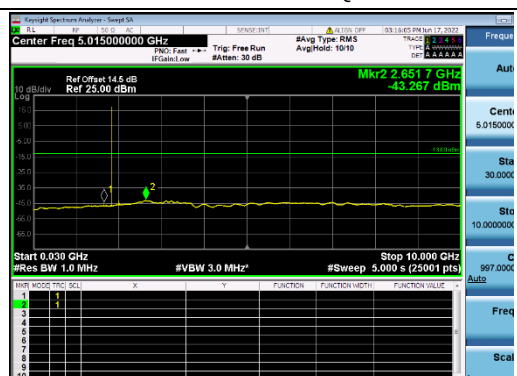
B25-15M-Low CH-CSE-2-QPSK-1 RB 0
