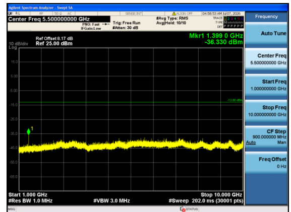
Band12-3MHz-QPSK-23025-1#0-1000-10000-PASS
