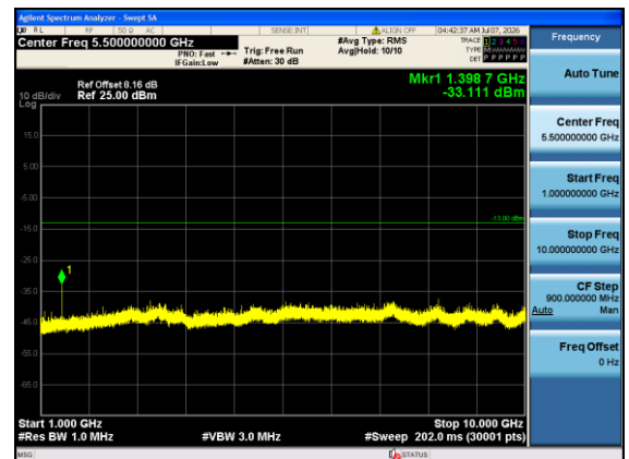
Band12-1.4MHz-QPSK-23017-1#0-1000-10000-PASS
