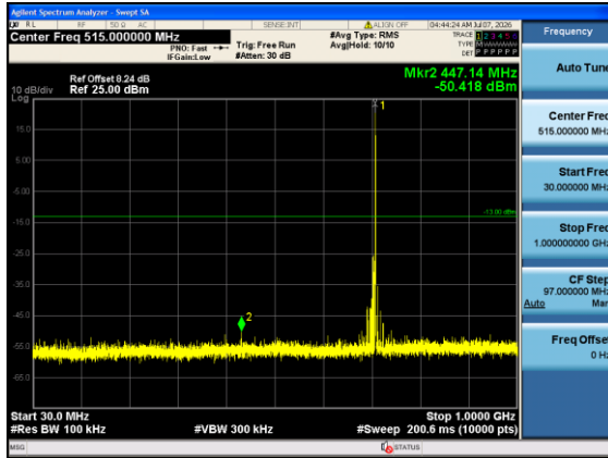
Band12-1.4MHz-QPSK-23173-1#5-30-1000-PASS
