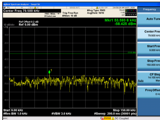
Band12-3MHz-QPSK-23095-1#0-0.009-0.15-PASS
