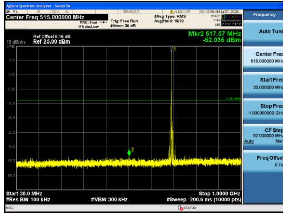
Band12-1.4MHz-16QAM-23017-1#0-30-1000-PASS
