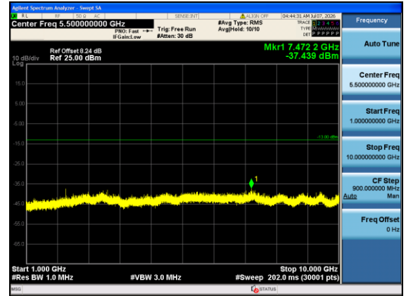
Band12-1.4MHz-QPSK-23173-1#5-1000-10000-PASS
