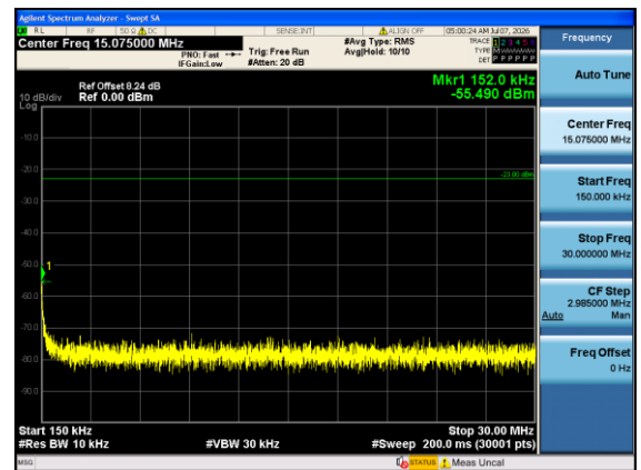
Band12-3MHz-QPSK-23165-1#5-0.15-30-PASS
