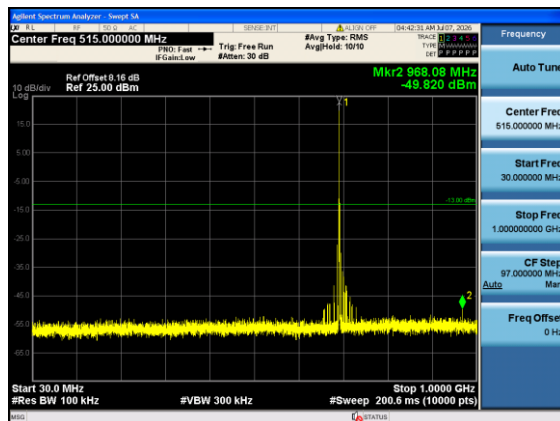
Band12-1.4MHz-QPSK-23017-1#0-30-1000-PASS
