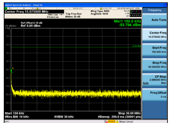
Band12-1.4MHz-16QAM-23017-1#0-0.15-30-PASS
