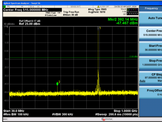
Band12-3MHz-16QAM-23025-1#0-30-1000-PASS
