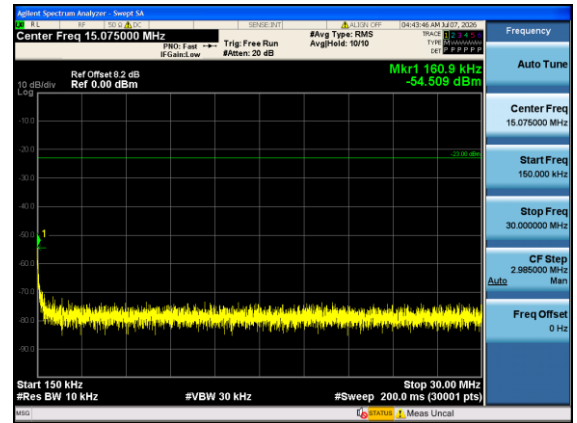
Band12-1.4MHz-16QAM-23095-1#0-0.15-30-PASS
