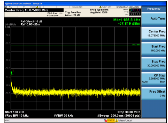
Band12-1.4MHz-QPSK-23017-1#0-0.15-30-PASS
