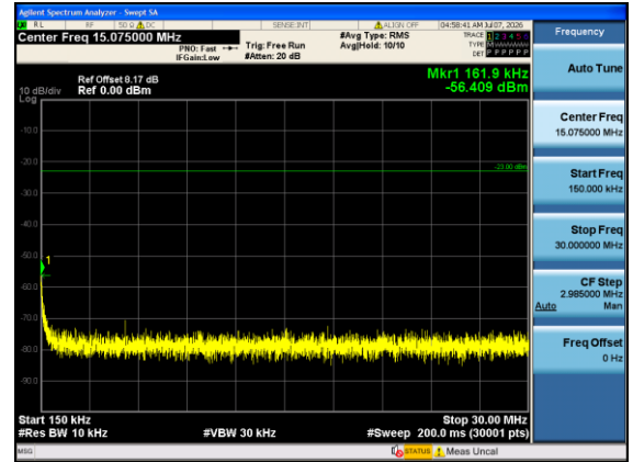
Band12-3MHz-QPSK-23025-1#0-0.15-30-PASS
