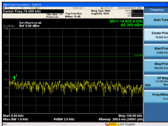
Band12-1.4MHz-16QAM-23173-1#5-0.009-0.15-PASS
