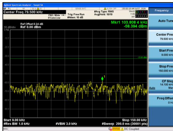
Band12-3MHz-QPSK-23165-1#5-0.009-0.15-PASS
