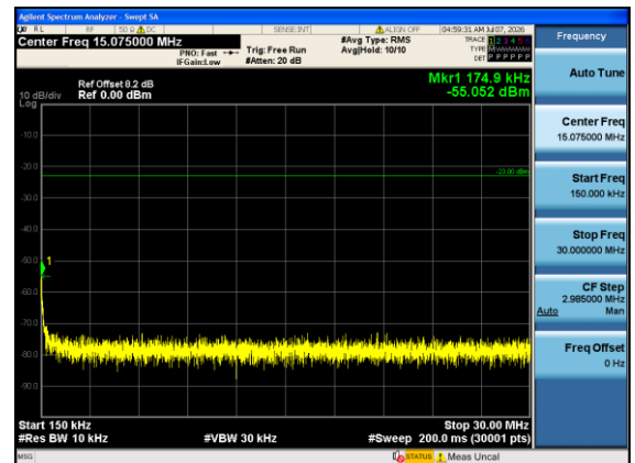
Band12-3MHz-QPSK-23095-1#0-0.15-30-PASS
