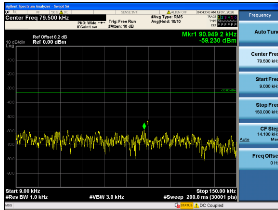
Band12-1.4MHz-16QAM-23095-1#0-0.009-0.15-PASS
