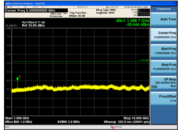
Band12-3MHz-16QAM-23025-1#0-1000-10000-PASS
