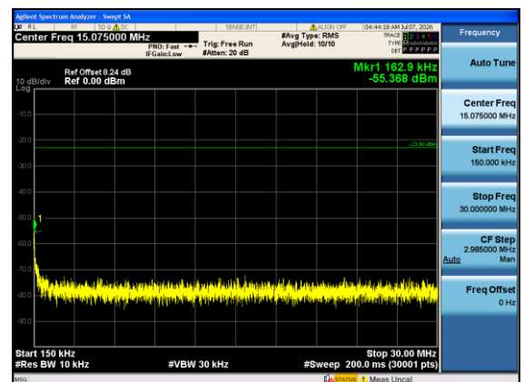
Band12-1.4MHz-QPSK-23173-1#5-0.15-30-PASS
