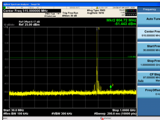
Band12-3MHz-QPSK-23025-1#0-30-1000-PASS
