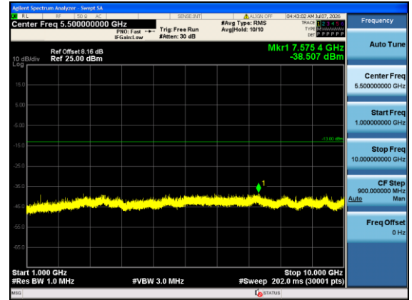
Band12-1.4MHz-16QAM-23017-1#0-1000-10000-PASS
