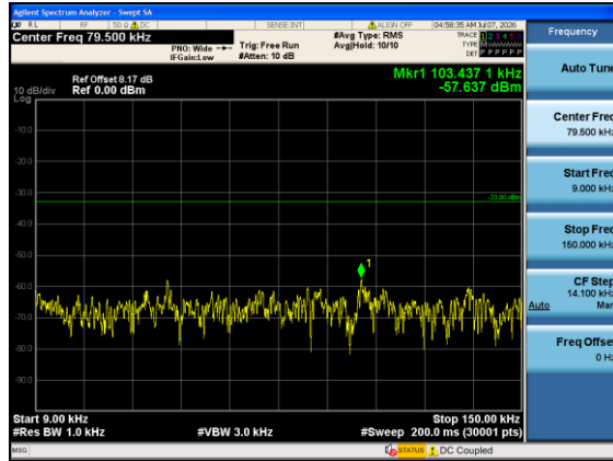
Band12-3MHz-QPSK-23025-1#0-0.009-0.15-PASS
