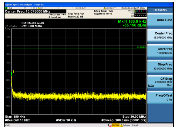
Band12-1.4MHz-16QAM-23173-1#5-0.15-30-PASS
