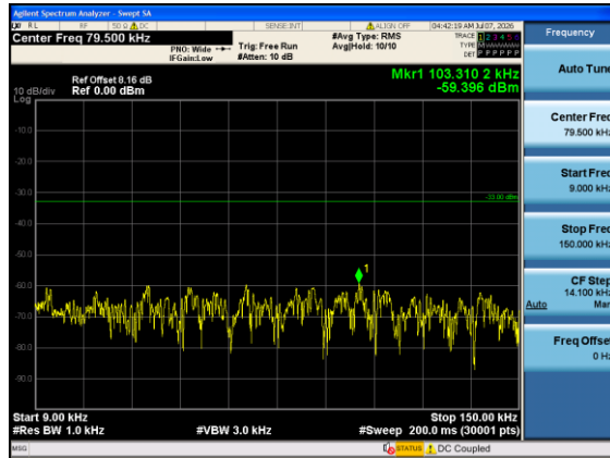
Band12-1.4MHz-QPSK-23017-1#0-0.009-0.15-PASS
