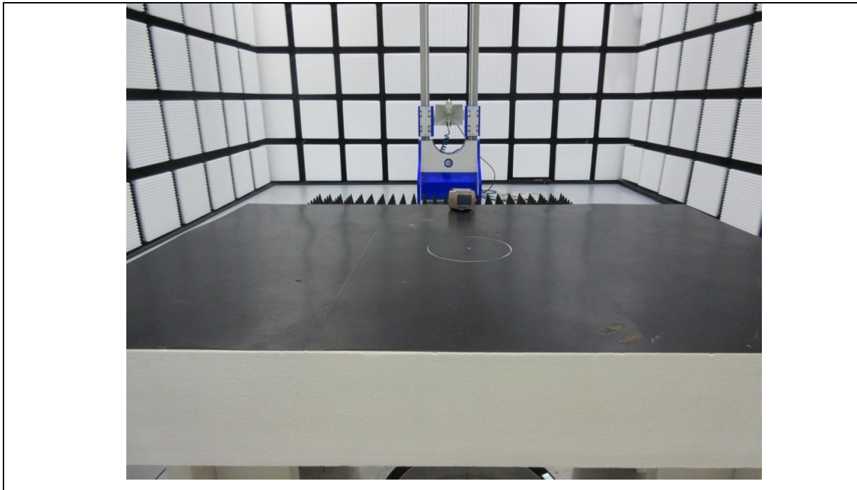
Radiated Emission Test (above 1G)
