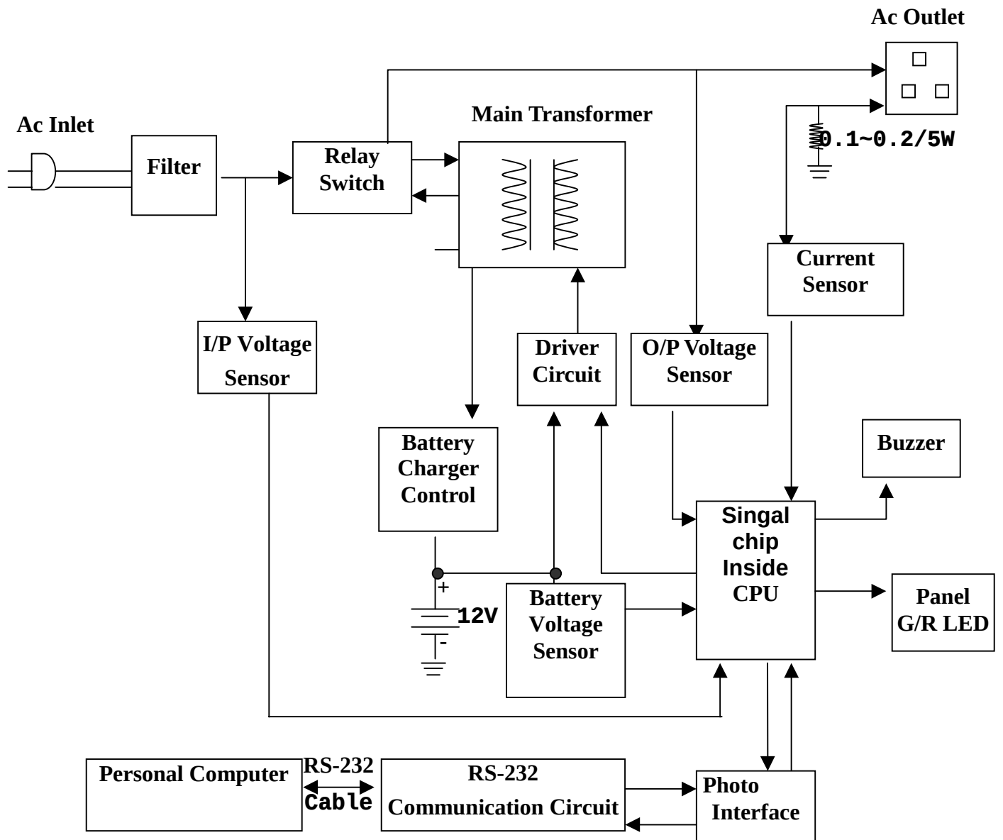
*** VT525P/625P Circuit Block Diagram ***
