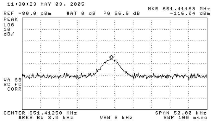
Figure 6.1. Relative receiver emissions in stand-by and activated modes. The final emission measurements were made with the receiver in activated mode.
