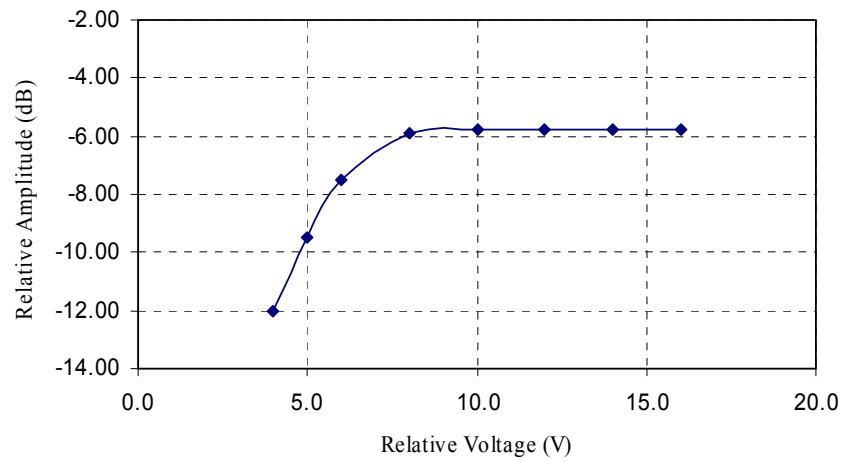
Figure 6.4. Relative emission at 125 kHz vs. supply voltage.
