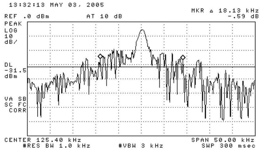
Figure 6.3. Measured bandwidth of the DUT. (pulsed)
