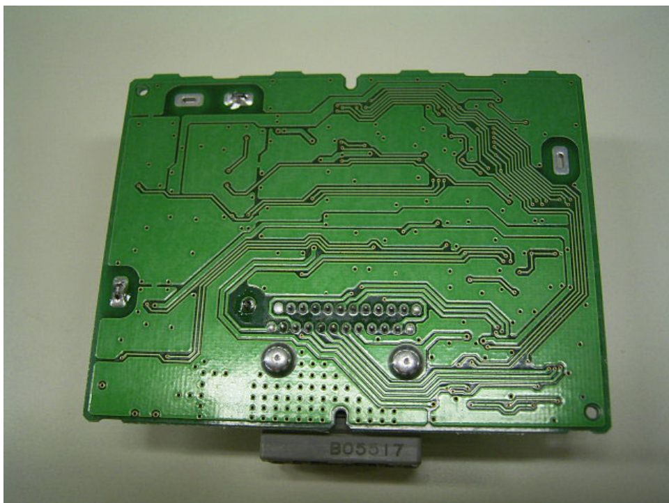
Figure 7.4 PCB assy (back view)
