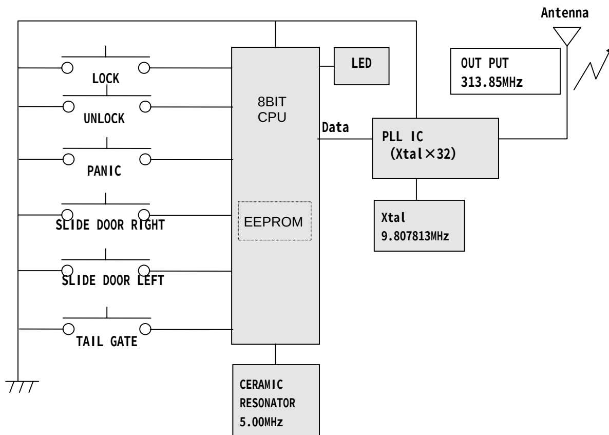
Figure 3.1 block diagram of the transmitter
