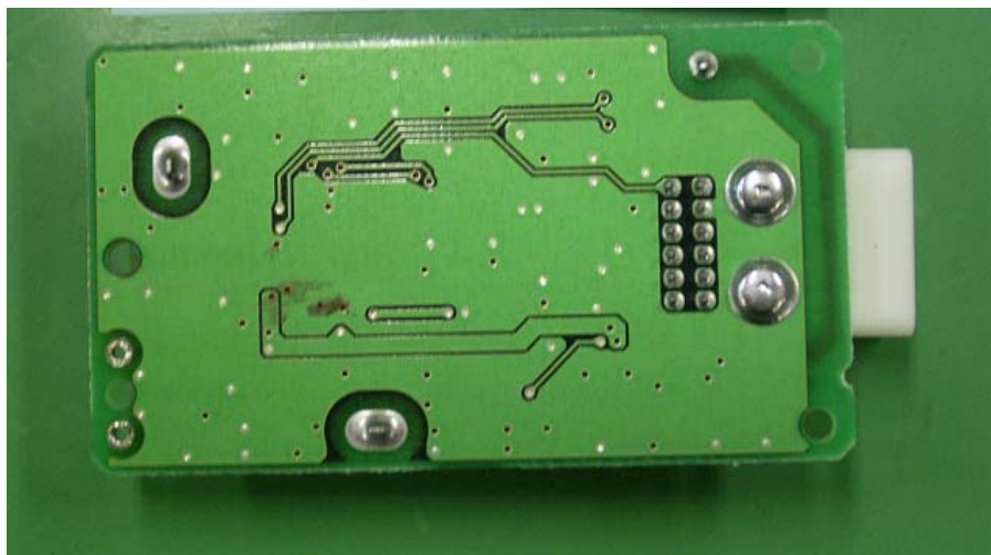
Figure 8.8 G8D-640M-RAM-N PCB assy (back view)
