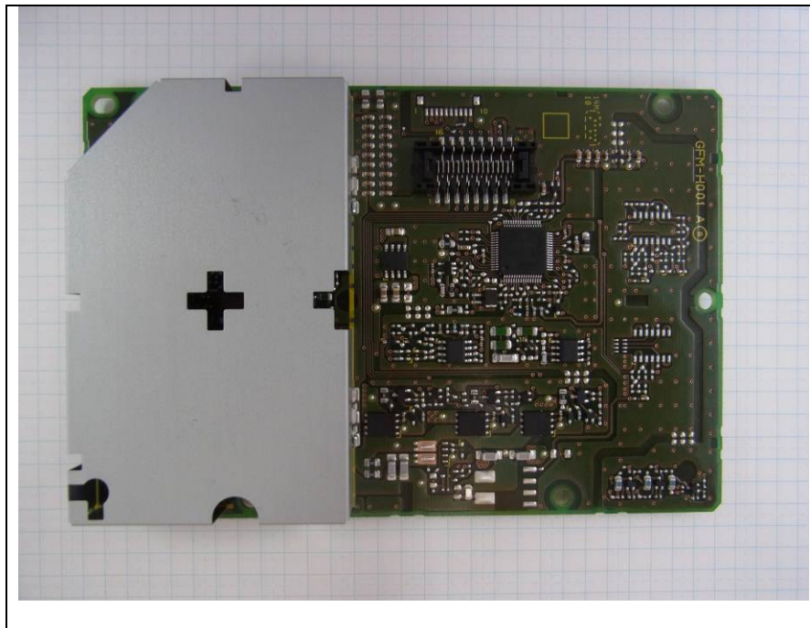
Figure 8.8 Wireless Charger Module with Shield [6] [9](bottom view)
