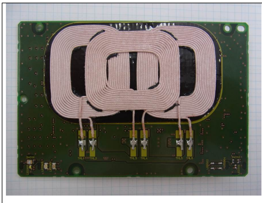
Figure 8.7 Wireless Charger Module [6] (bottom view)
