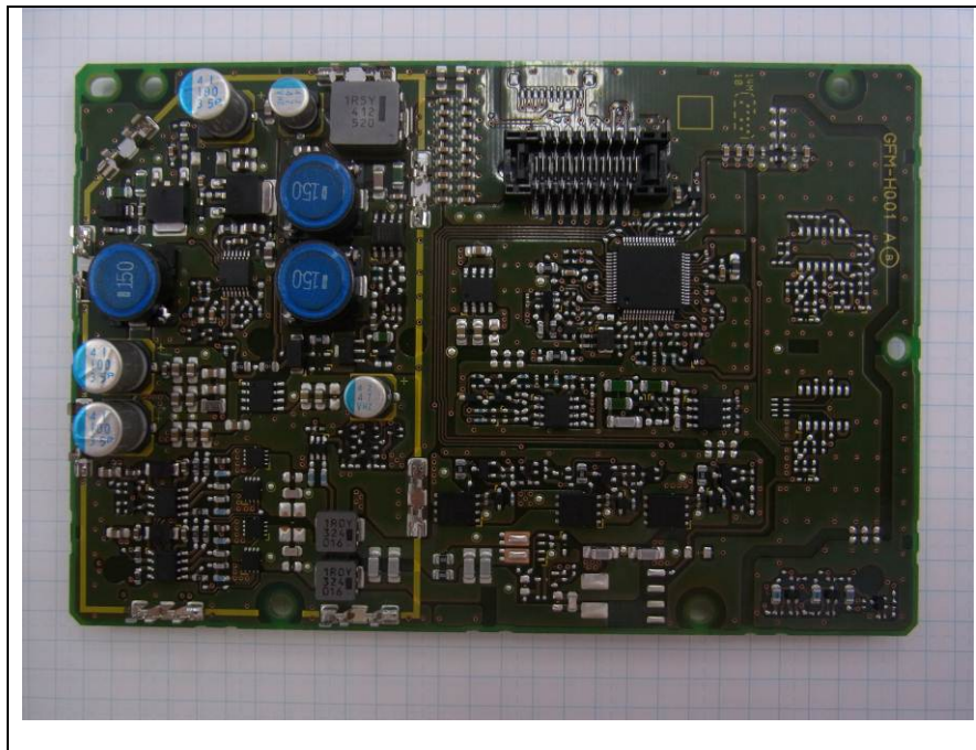
Figure 8.6 Wireless Charger Module [6] (top view)
