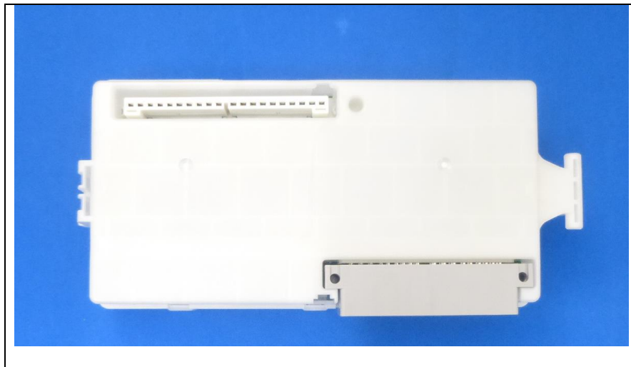
Figure 7.1 Appearance (front view)
