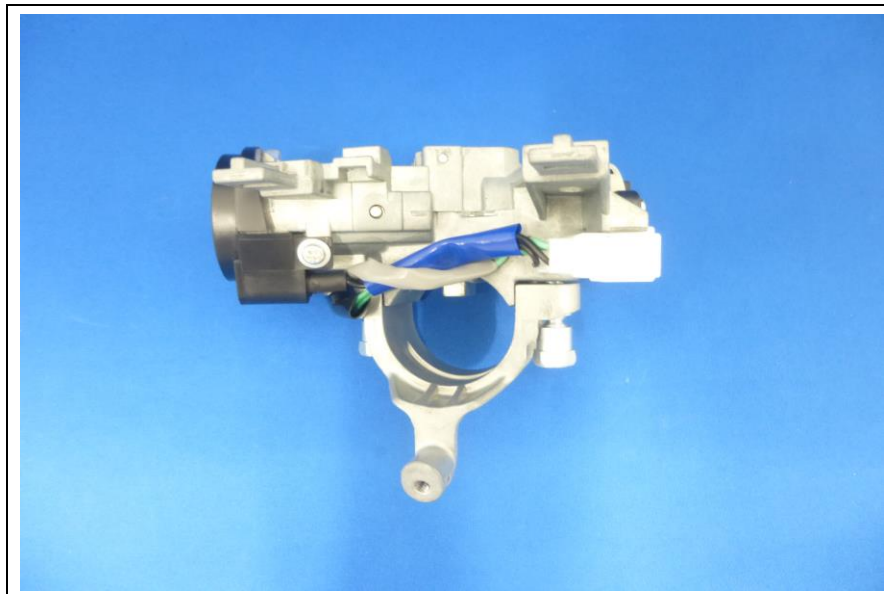
Figure 7.10 Antenna Coil (External2 view)
