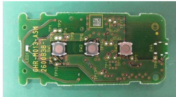
Figure 8.1 FOB appearance (PCB [Basic]) Front
