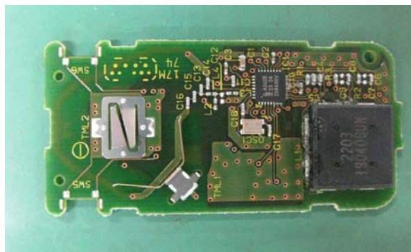
Figure 8.2 FOB appearance (PCB [Basic]) Back
