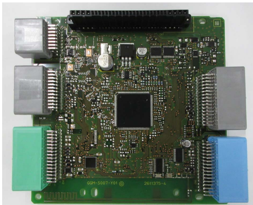
Figure 8.1 K56RA PCB assy (top view)
