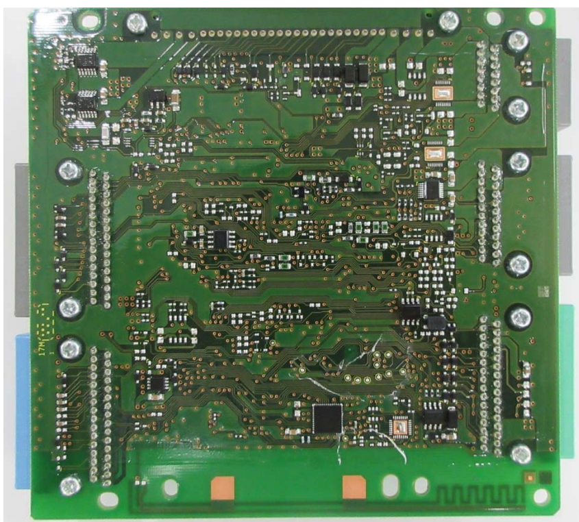
Figure 8.1 K56RA PCB assy (top view)
