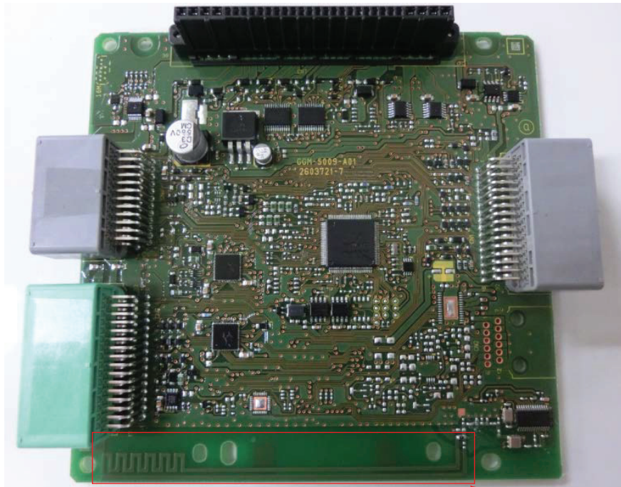
Antenna (Rx)
