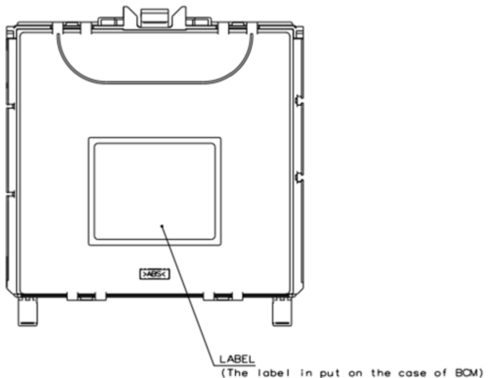
Figure 9.2 K56RQ appearance
