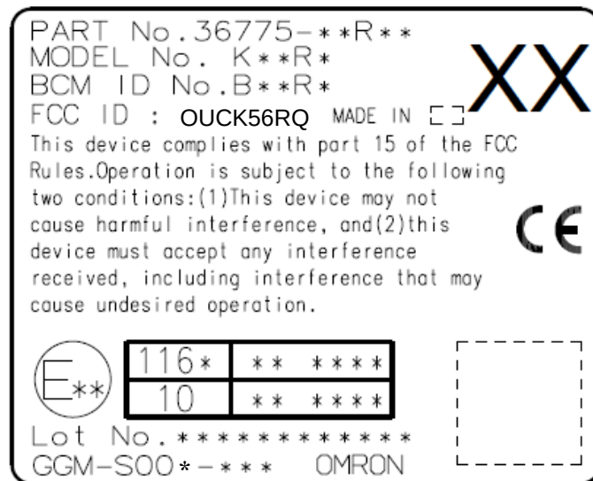
Figure 9.1 K56RQ Label
