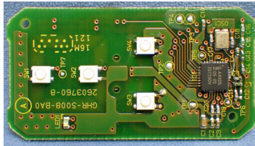
Figure 8.7 PCB assy (front view)
