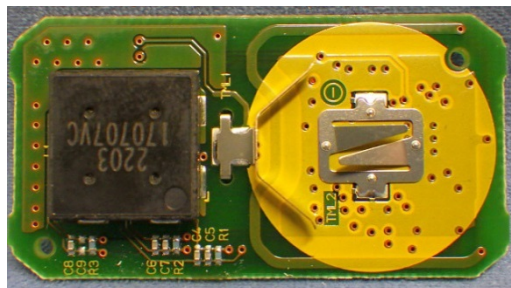
Figure 8.8 PCB assy (back view)
