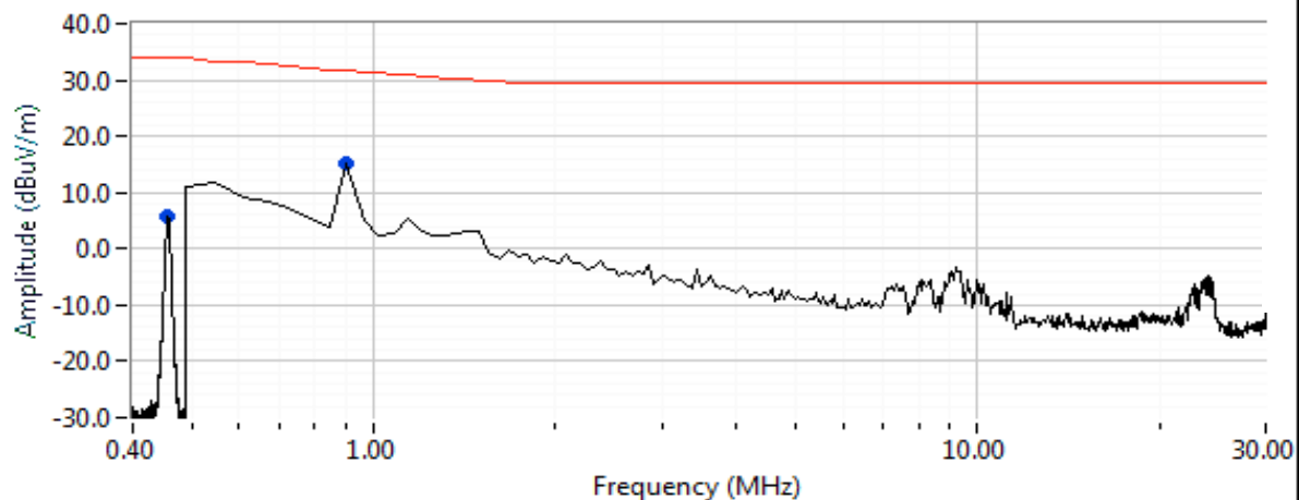
Run #3: EUT flat (Antenna Closed side)
