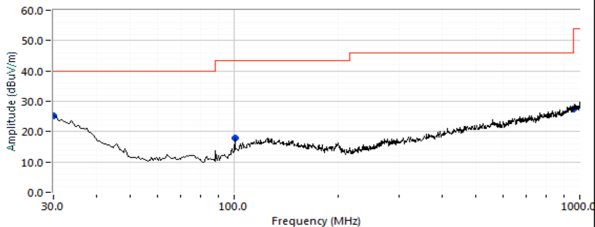
Run #1: 30 - 1000 MHz
