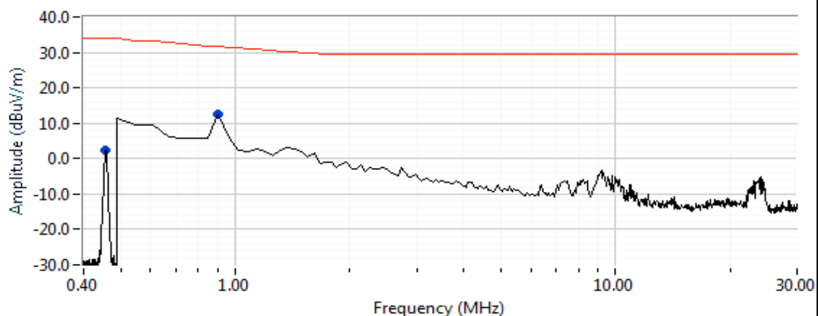
Run #3: EUT on side (Antenna Closed)
