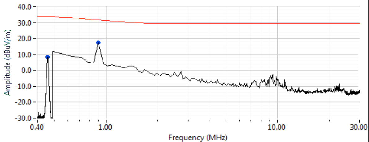
Run #3: EUT flat (Antenna Open)
