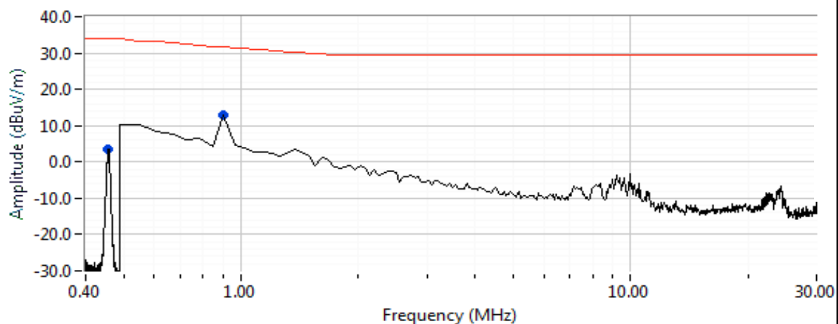
Run #3: EUT upright (Antenna Closed side)
