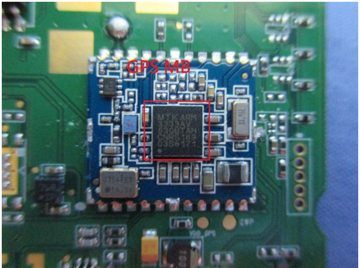
(26) EUT Photo (GPS (MB)
