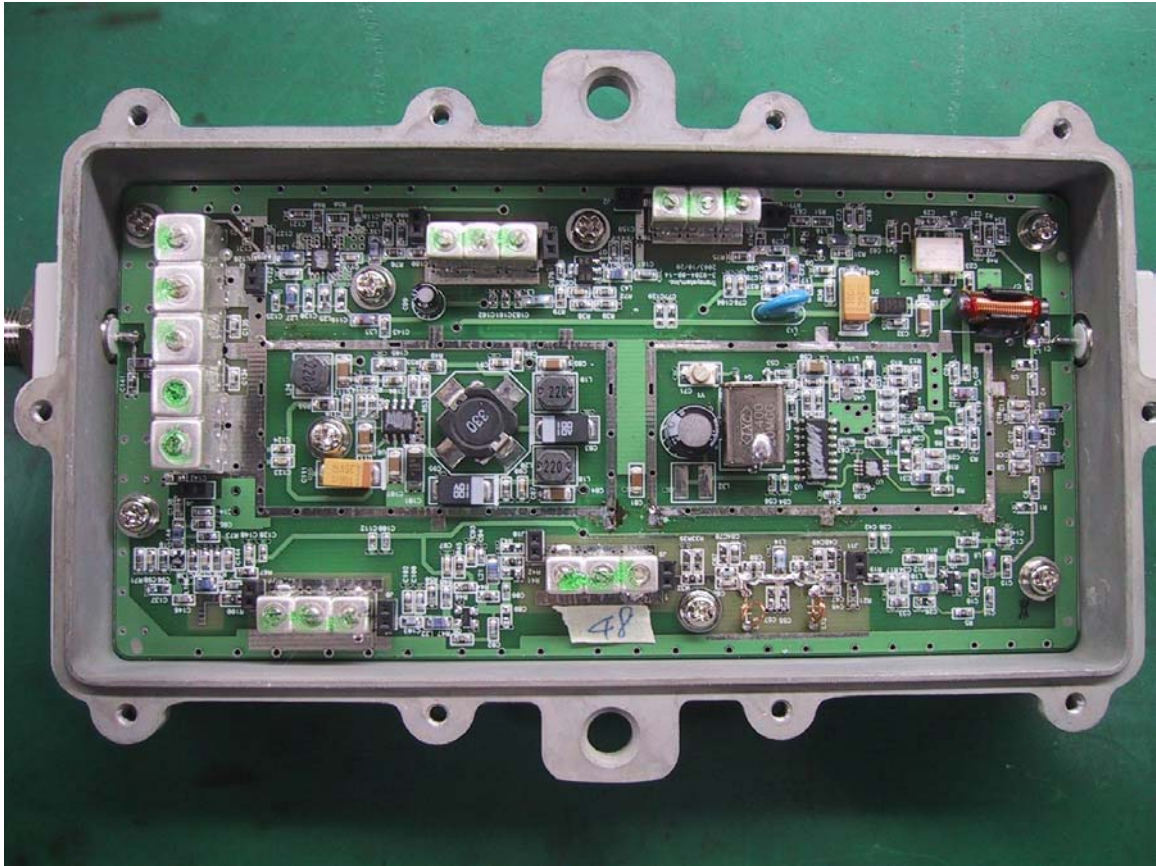
Interior, no shields
