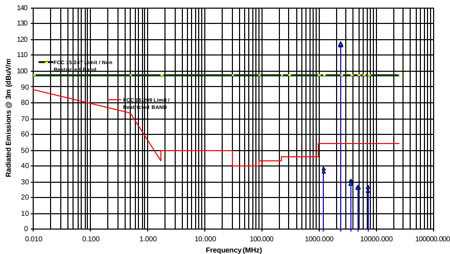
Transmitter Radiated Emissions Measurements at 3 Meter OFTS MAXSTREAM MODEL 24XSTREAM Tx Freq.: 2404.48 MHz (Lowest) with Model A24-HABSM 1/2 Dipole Antenna
