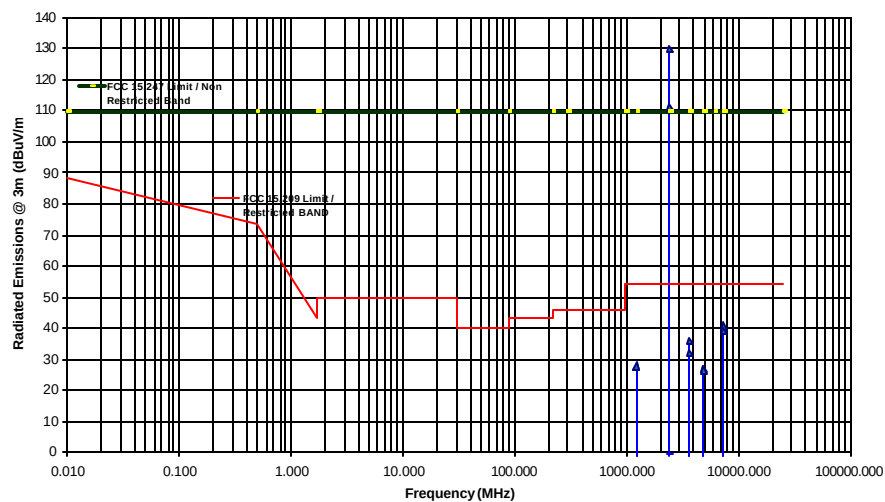
Transmitter Radiated Emissions Measurements at 3 Meter OFTS MAXSTREAM MODEL 24XSTREAM TRANSMIT Freq.: 2443.75 MHz (Middle) with Model A24-Y18RM Yagi Directional Antenna
