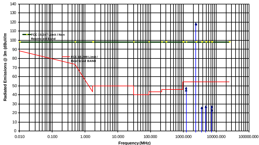
Transmitter Radiated Emissions Measurements at 3 Meter OFTS MAXSTREAM MODEL 24XSTREAM Tx Freq.: 2443.75 MHz (Middle) with Model A24-HABSM 1/2 Dipole Antenna
