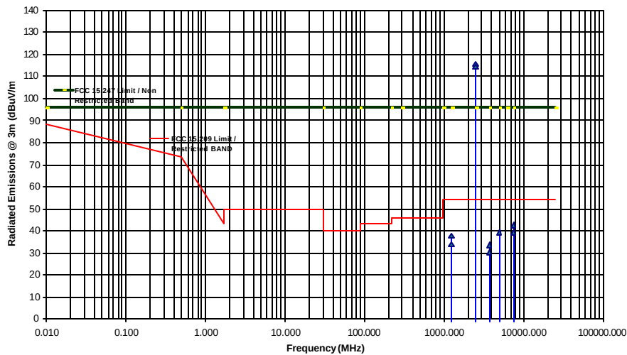
Transmitter Radiated Emissions Measurements at 3 Meter OFTS MAXSTREAM MODEL 24XSTREAM Tx Freq.: 2482.15 MHz (Middle) with Model A24-HABSM 1/2 Dipole Antenna
