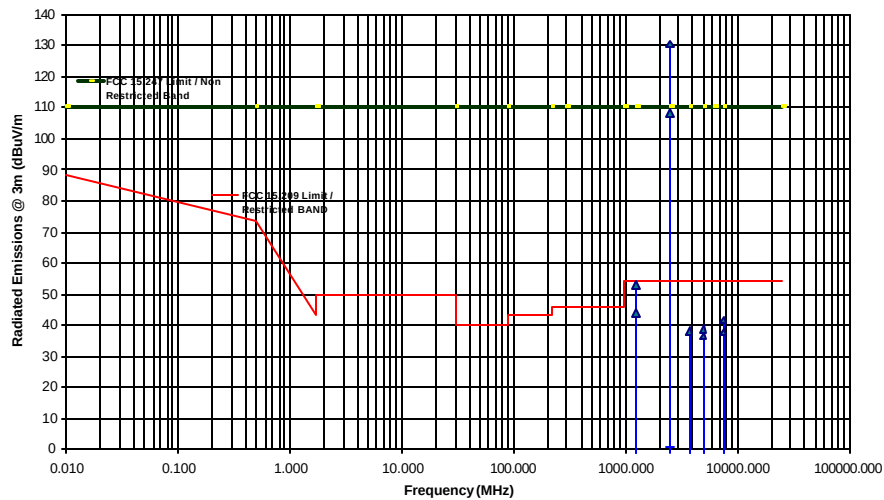
Transmitter Radiated Emissions Measurements at 3 Meter OFTS MAXSTREAM MODEL 24XSTREAM Tx Freq.: 2482.15 MHz (Middle) with Model Model A24-P19RM Flat Panel Antenna
