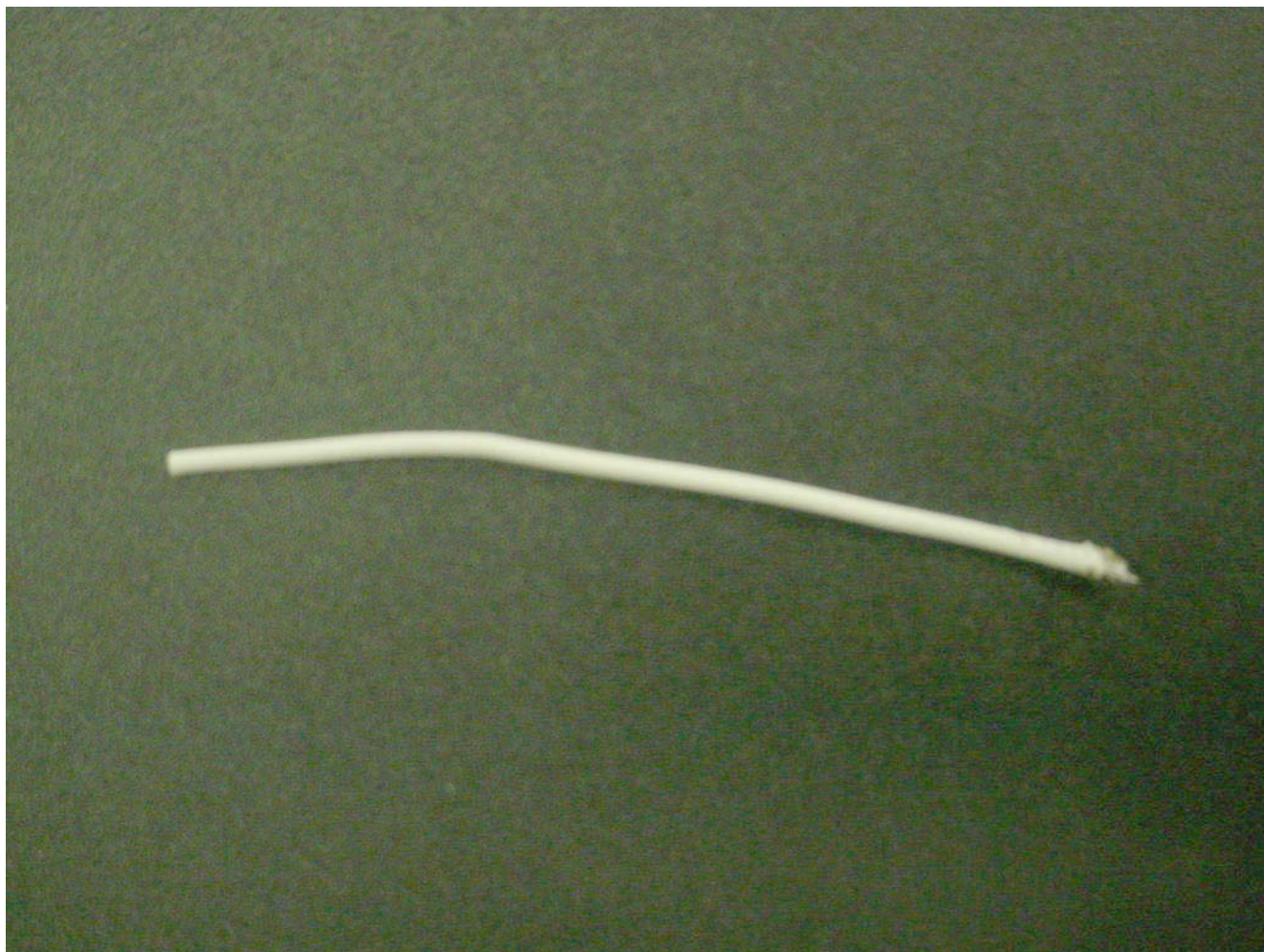
Monopole Antenna (A09-QW, 1.9dBi Quarter-wave wire antenna, Permanent)
