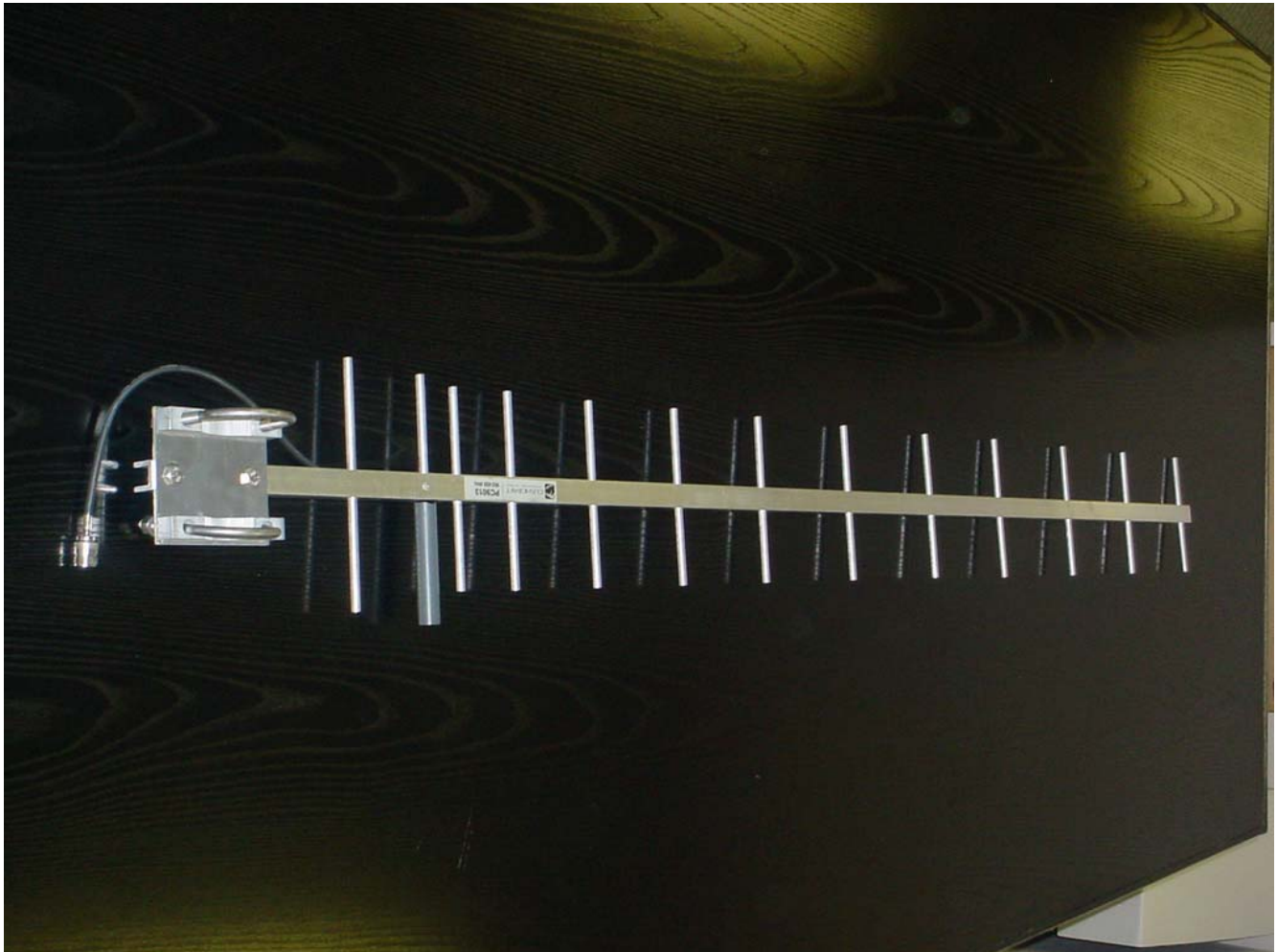
Yagi Antenna (A09-Y15TM, 15.1dBi gain 13 element Yagi antenna, RPTNC)
