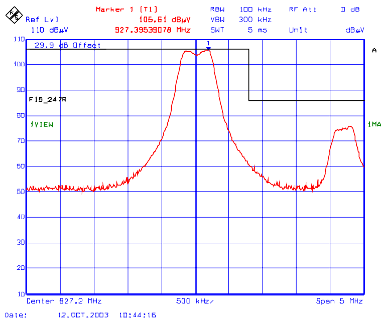
Plot 74: Band-edge Radiated Emissions @ 3 Meters (FHSS Mode) Vertical Polarization
