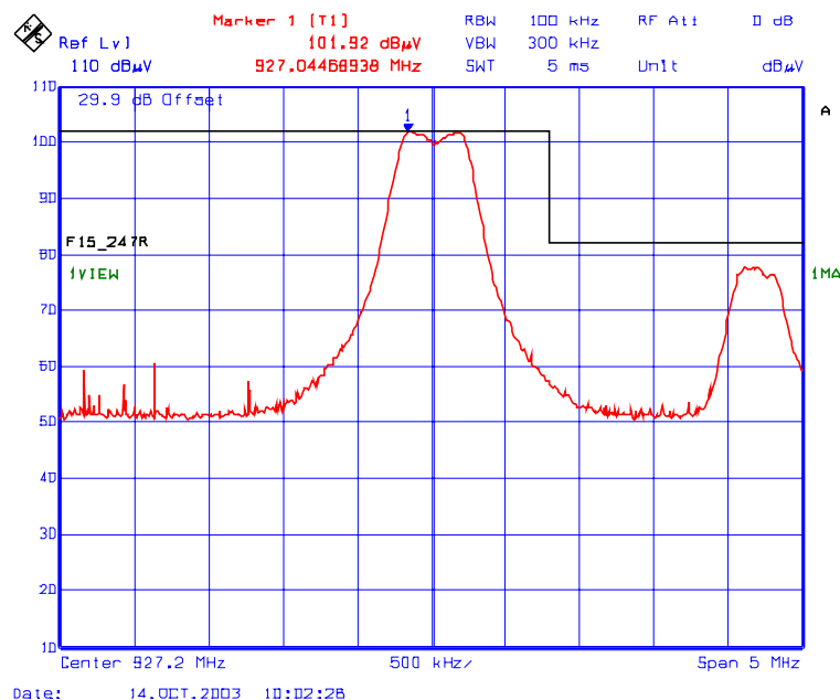
Plot 42: Band-edge Radiated Emissions @ 3 Meters (FHSS Mode) Vertical Polarization
