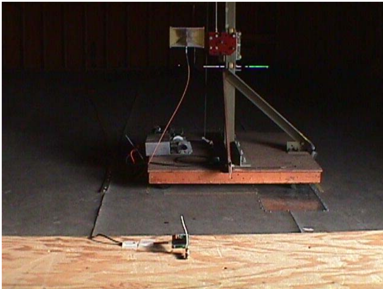
Radiated Emissions @ 3 Meters EUT with Monopole Antenna (A09-QW, 1.9dBi Quarter-wave wire antenna, Permanent)
