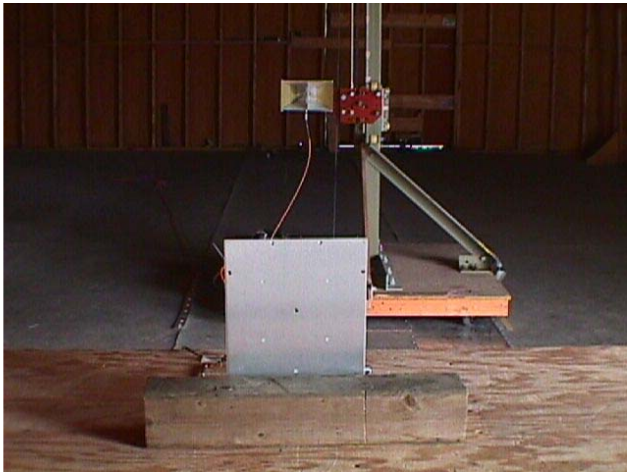
Radiated Emissions @ 3 Meters EUT with Panel Antenna (A09-P8TM, 8dBi Panel antenna, RPTNC)
