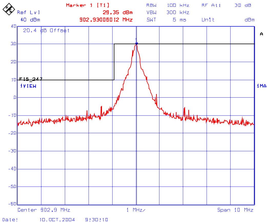
Plot 17: Band-Edge RF Conducted Emissions Low End of Frequency Band Single Frequency Mode
